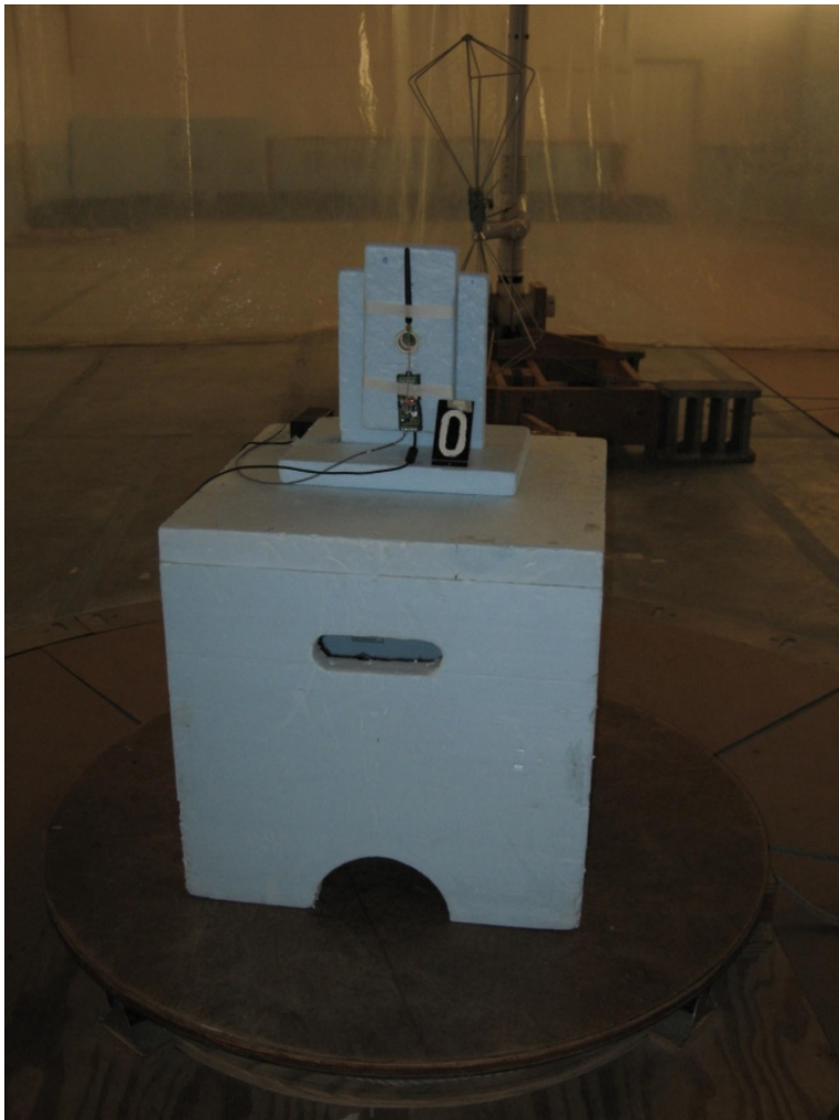
Model 11-115-0001 Radiated Front - Below 1 GHz
