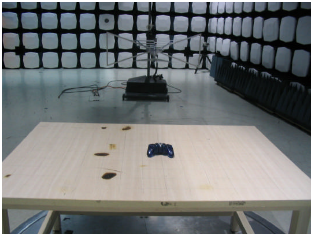
Setup Photo-2
