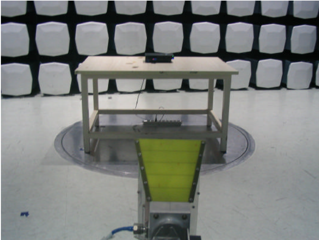
Setup Photo-5
