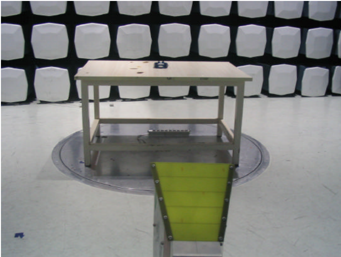
Setup Photo-4
