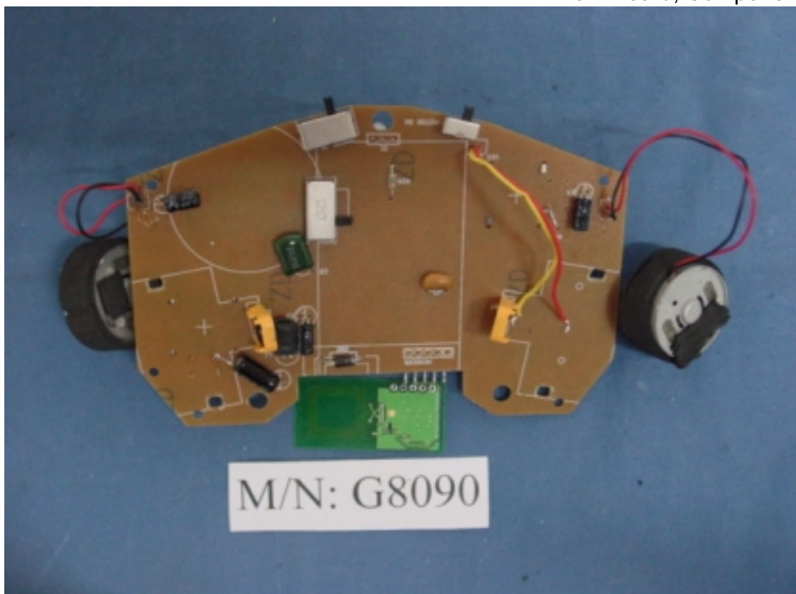
Figure 9 Main Board, Component Side
