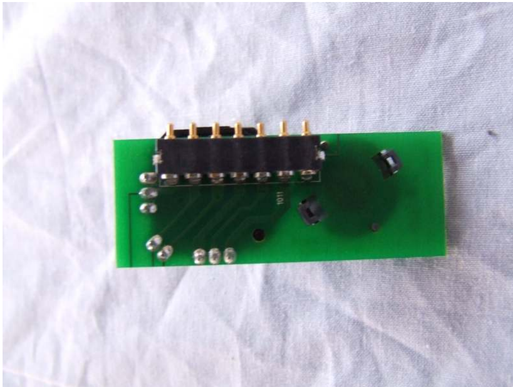
Photo 5-Back view of Button Board
