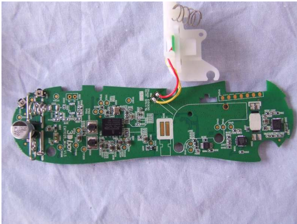
Photo 2-Front view of RF Main Board
