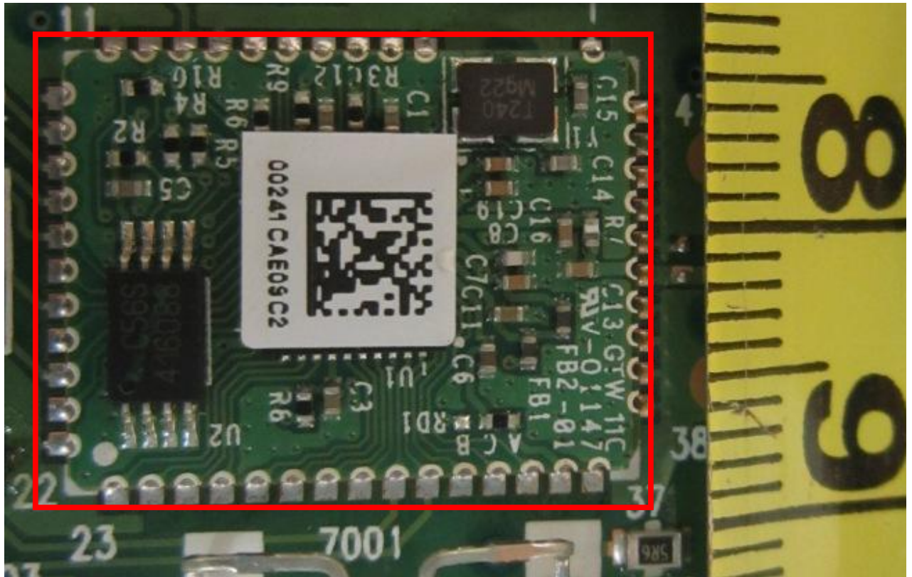
RF Module Circuit with RF Shield Removed
