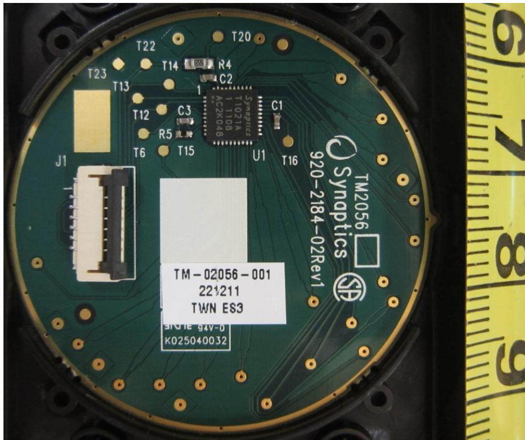
Sub-Board PCB Component Side
