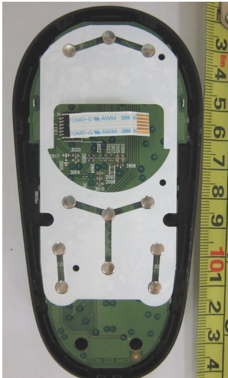
EUT Bottom Housing Internal View
