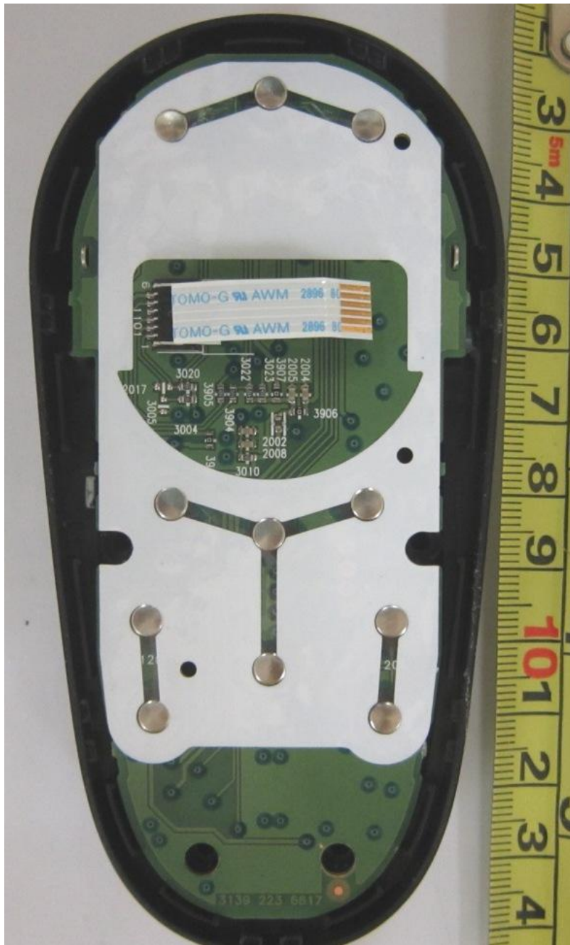
Main-Board PCB Component Side
