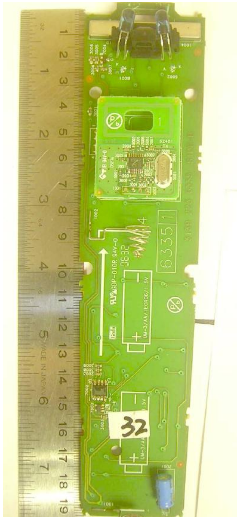
Main-Board - PCB Component Side
