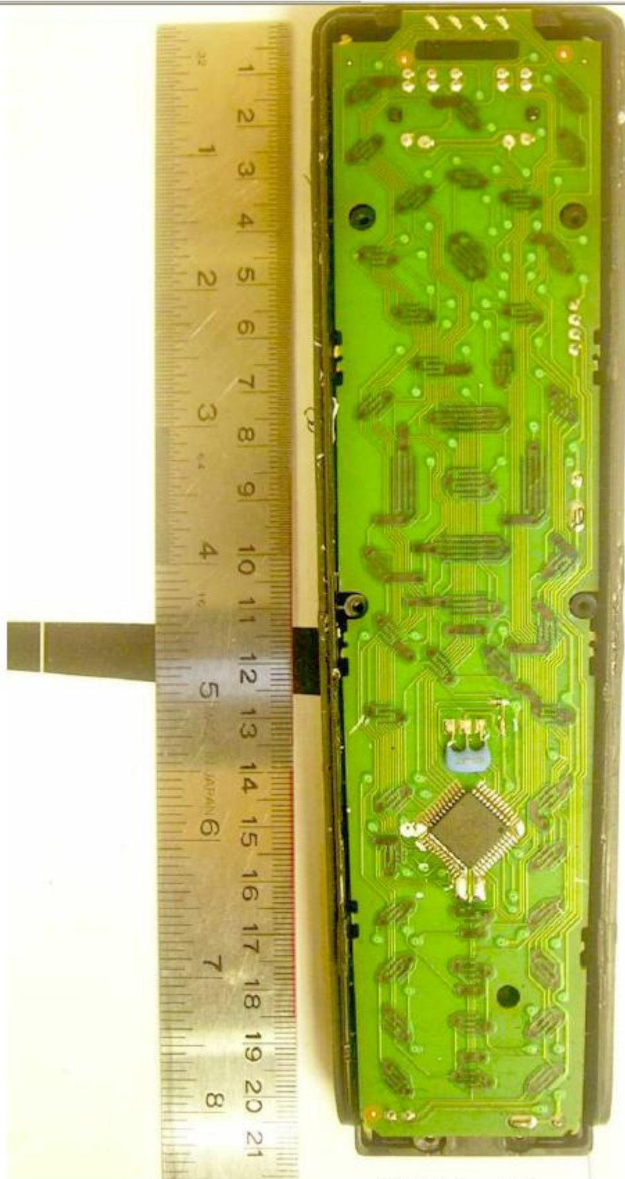
EUT Internal View
