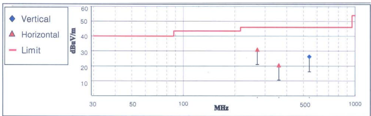
< Fig 5. Radiated emission result _ 90.1MHz >
