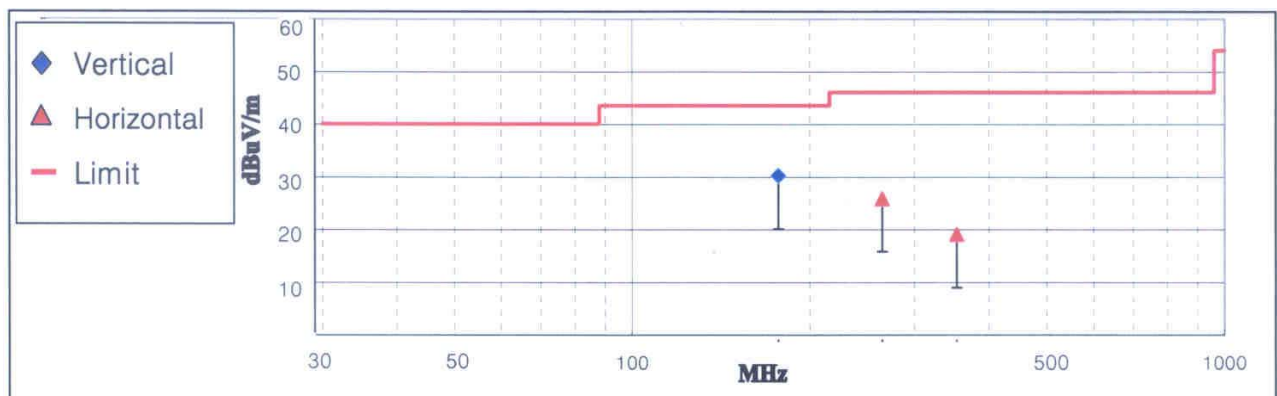
< Fig 4. Radiated emission result _ 88.3MHz >
