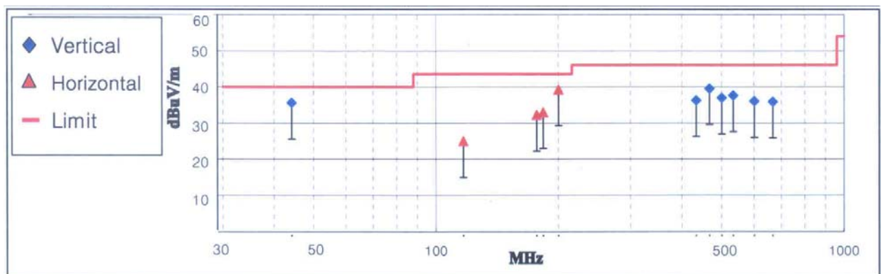
&lt; Fig 6. Radiated emission result _ Other frequency &gt;
