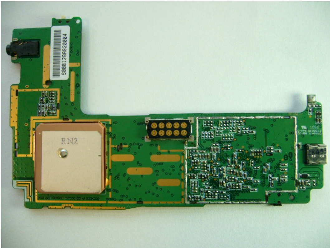
(17) EUT Photo (GPS Antenna : WAVEFAR-PTE86012)
