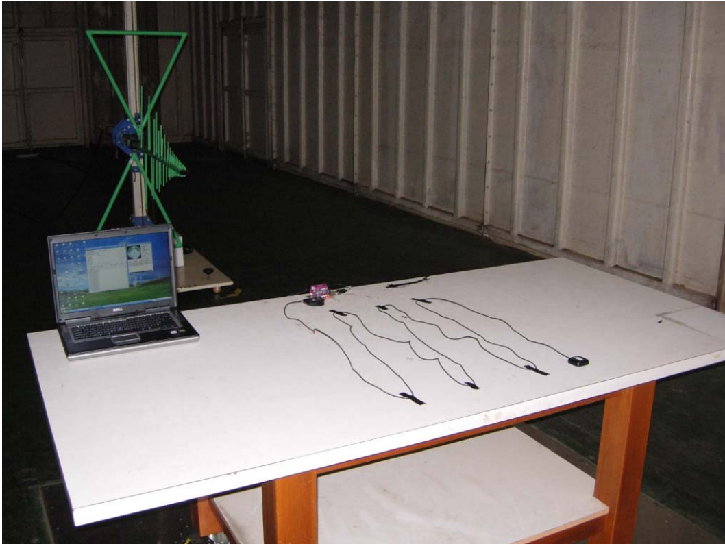
Back View of Radiated Test - Mode 1,5,9
