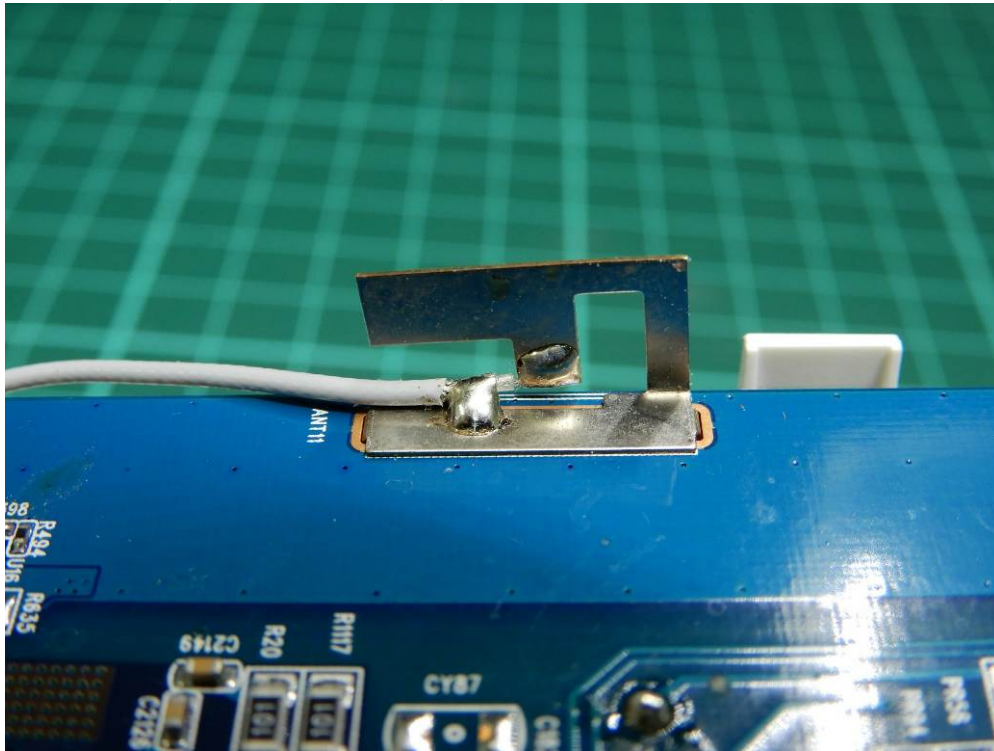
(11) EUT Photo (5GHz WLAN Antenna)
