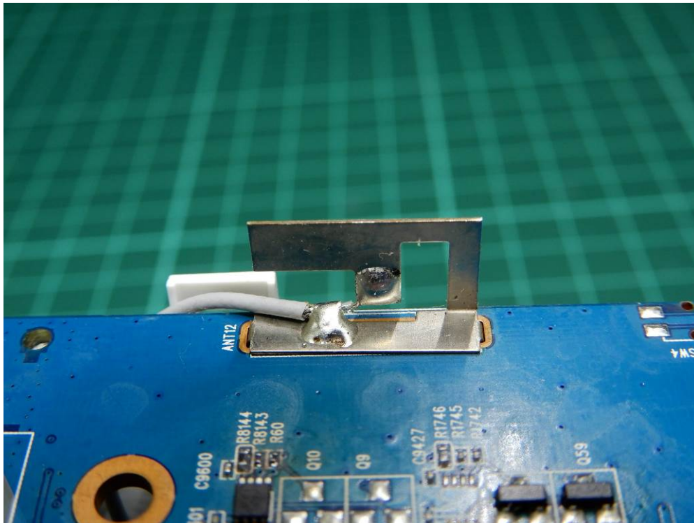
(12) EUT Photo (5GHz WLAN Antenna)
