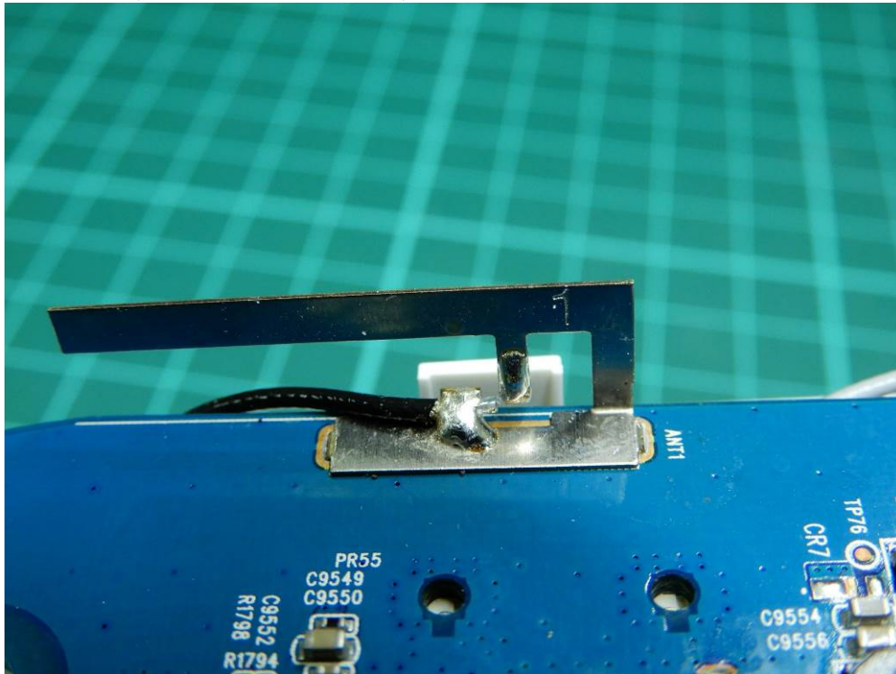
(9) EUT Photo (2.4GHz WLAN Antenna)
