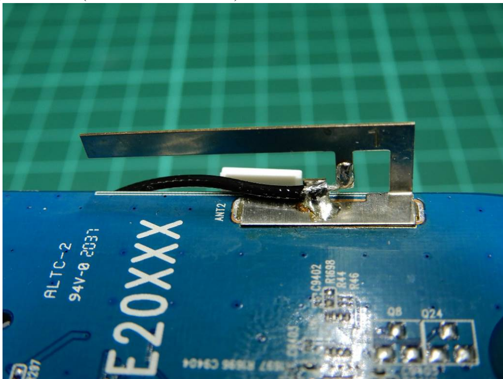
(10) EUT Photo (2.4GHz WLAN Antenna)
