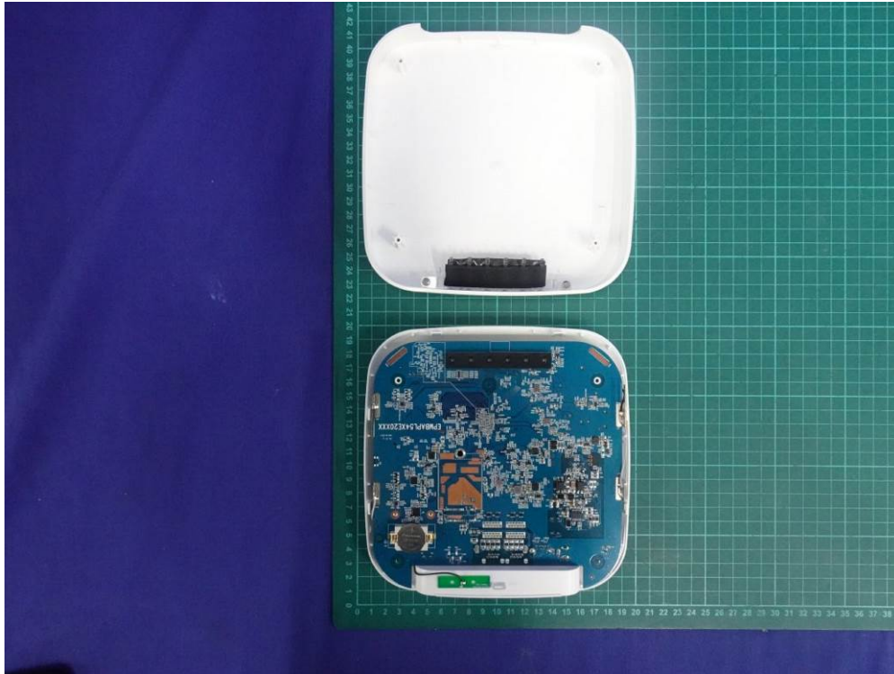
(1) EUT Photo (M/N: APL52X)
