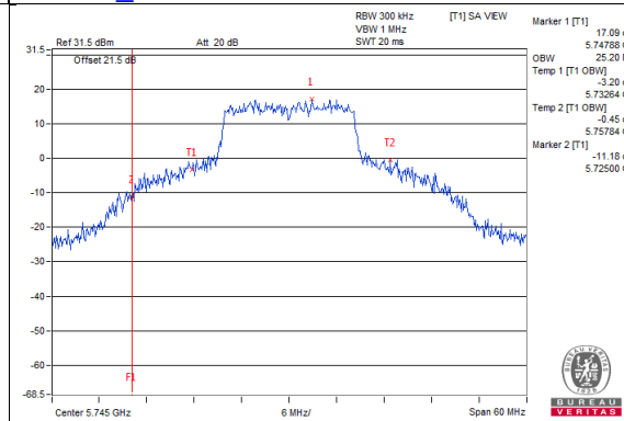
802.11ac(VHT20)_Chain1 / CH149
