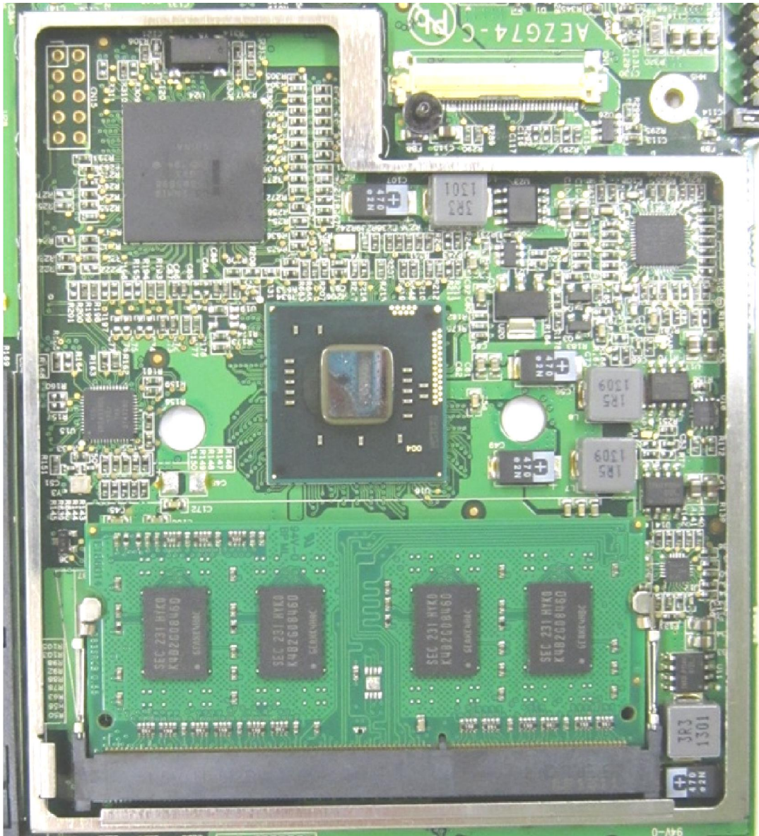
RAM-DDR3, CPU, Chipset with Shielding Removed
