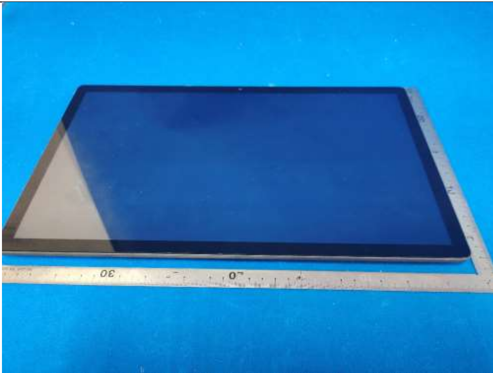
(5) EUT Photo(Model ESY1014)
