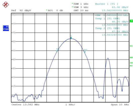
99% Bandwidth 13.56 MHz
