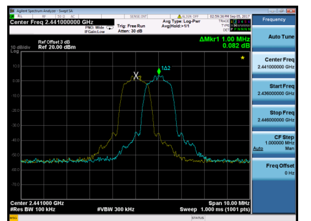
Channel 39 (2441MHz)
