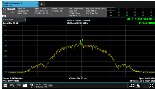
Modulation Type: GFSK(2Mbps) CH19
