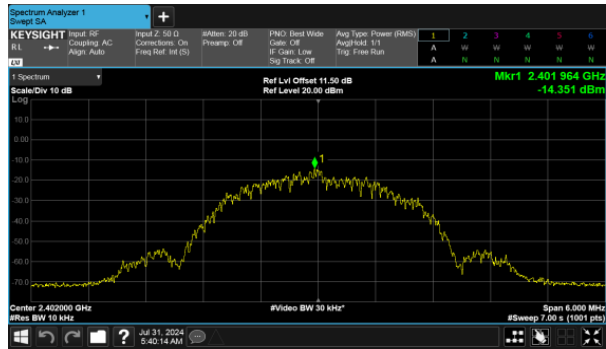
Modulation Type: GFSK(2Mbps) CH00
