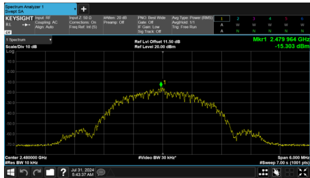
Modulation Type: GFSK(2Mbps) CH39
