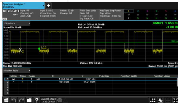
Modulation Type: GFSK-DH3
