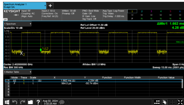
Modulation Type: AFH (DH3)
