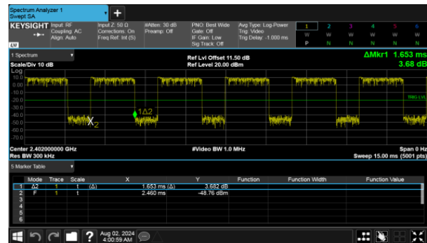
Modulation Type: \pi/4 -DQPSK-DH3
