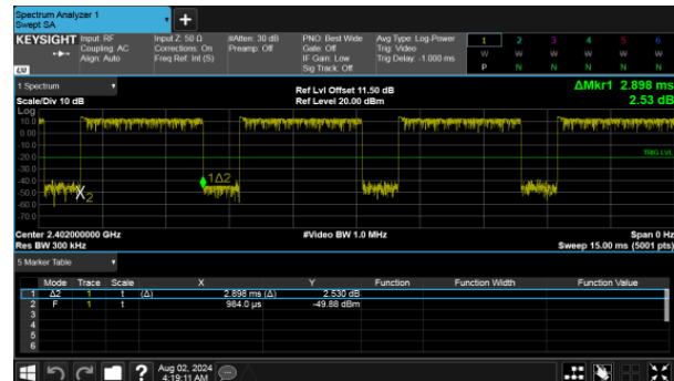
Modulation Type: \pi/4 -DQPSK-DH5 Channel: 00
