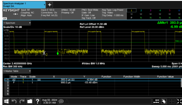
Modulation Type: GFSK-DH1 Channel: 00
