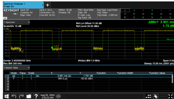
Modulation Type: AFH (DH5)
