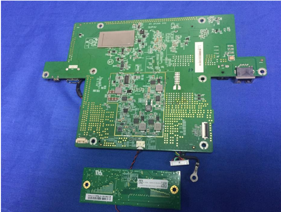
(7) EUT Photo
