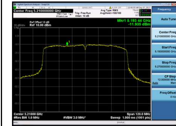
Channel 42 (5210MHz)
