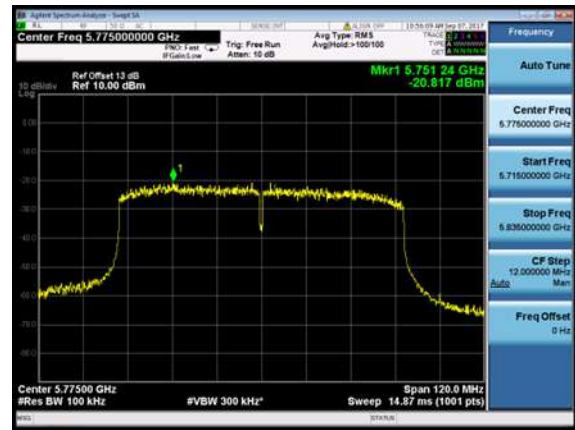
Channel 155 (5775MHz)
