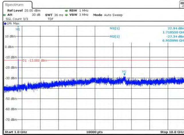
Band66-1.4MHz-QPSK-131979-1RB#0-Range2:1000~10000MHz
