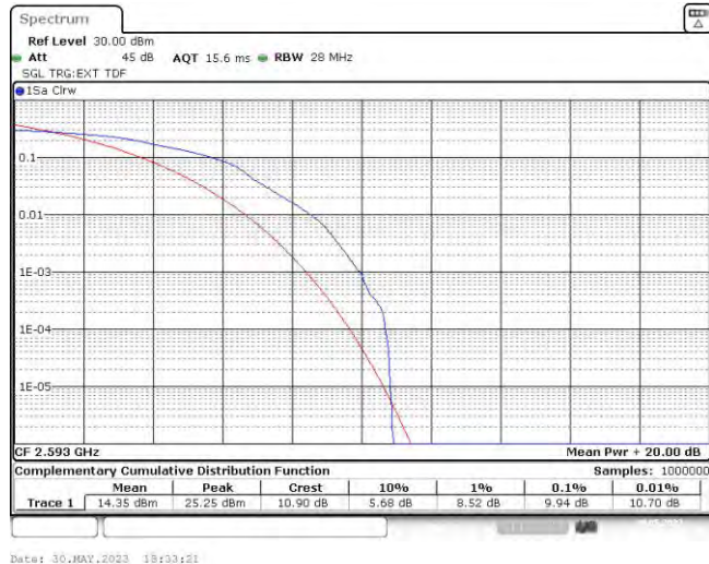
Band41-15MHz-16QAM-40620-75RB#0
