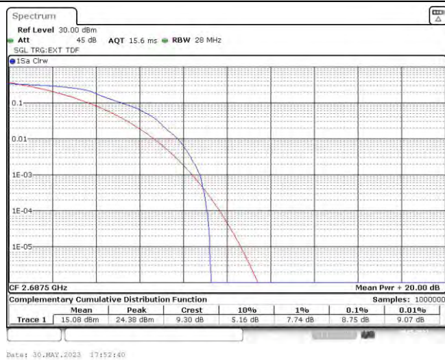
Band41-5MHz-QPSK-41565-25RB#0
