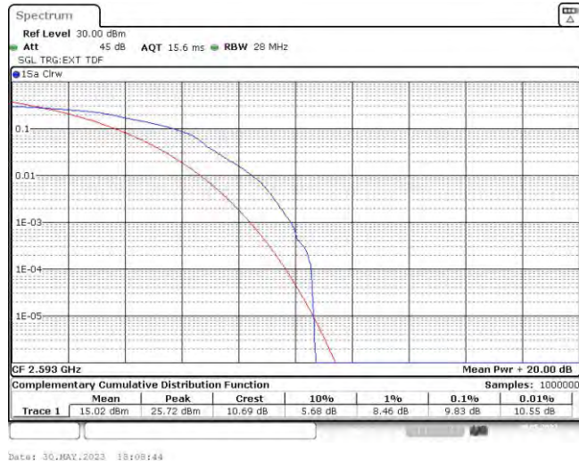
Band41-10MHz-16QAM-40620-50RB#0
