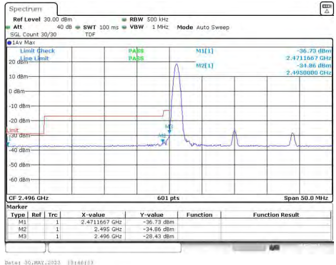
Band41-20MHz-16QAM-39750-1RB#99
