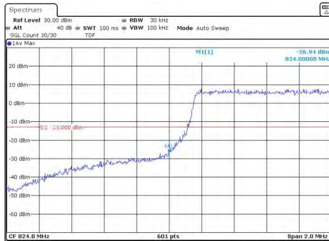
Band26-1.4MHz-16QAM-26797-6RB#0
