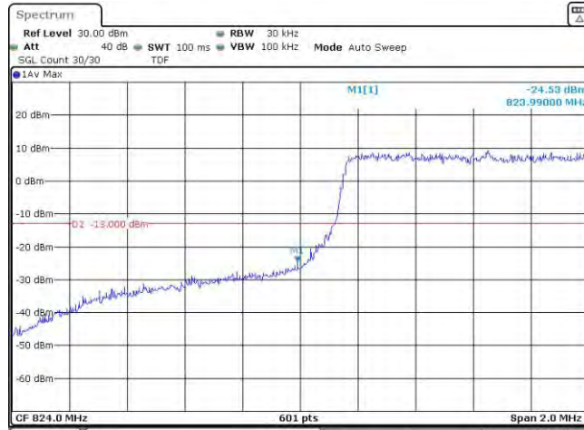
Band26-1.4MHz-QPSK-26797-6RB#0
