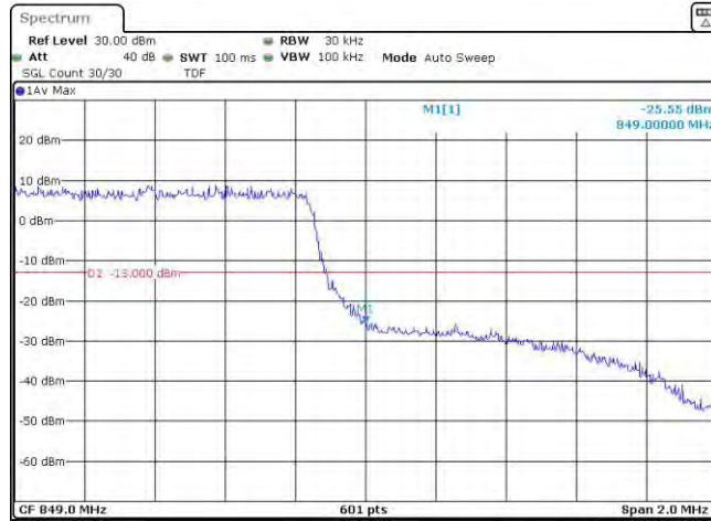
Band26-1.4MHz-QPSK-27033-6RB#0
