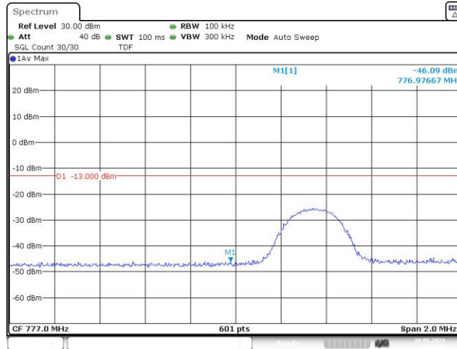
Band13-5MHz-QPSK-23205-1RB#24
