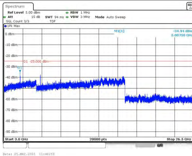
Band7-5MHz-QPSK-20775-25RB#0-Range3:3000~26500MHz
