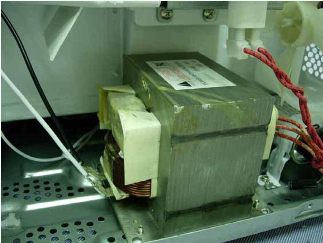
Photo 15 M/N: TSK-M3204ME, H.V. Transformer
