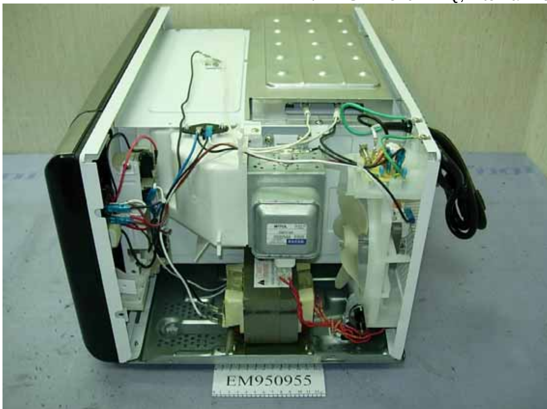
Photo 28 M/N: TSK-M3204MEQ, Internal View (Side)
