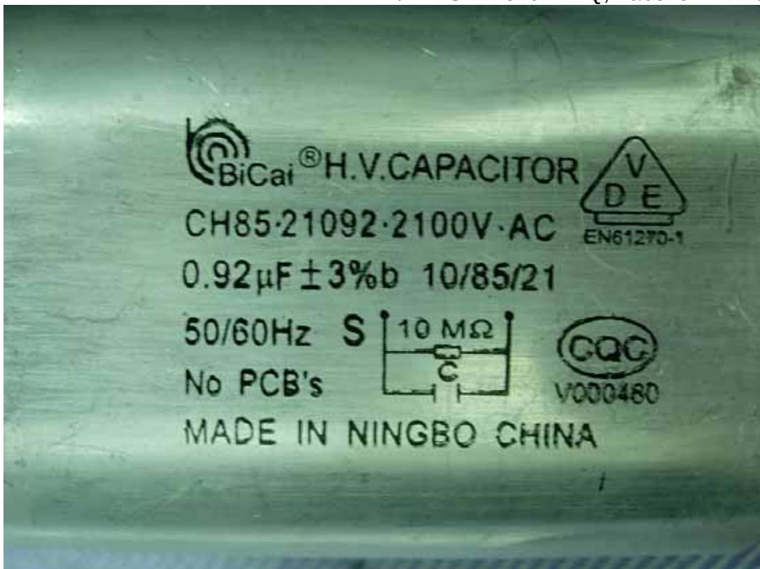
Photo 34 M/N: TSK-M3204MEQ, Label of H.V. Capacitor
