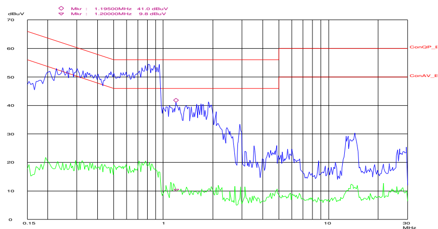
Line N Conducted Emission Graph
