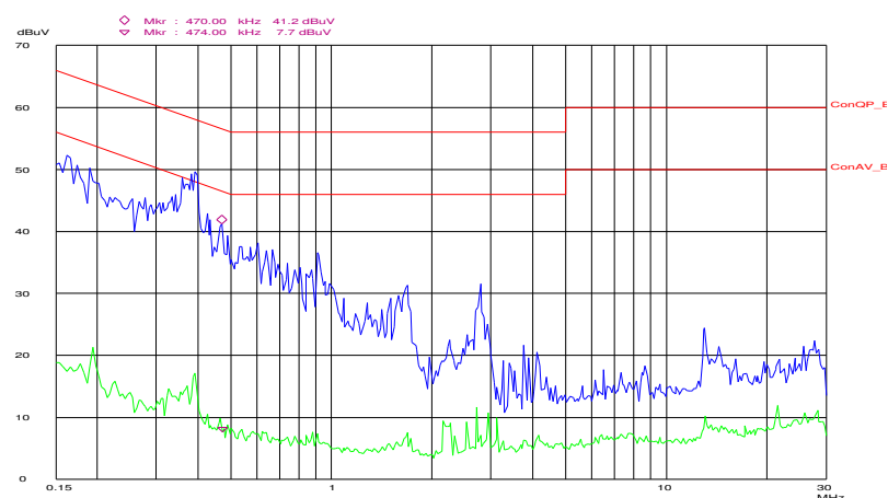
Line L Conducted Emission Graph
