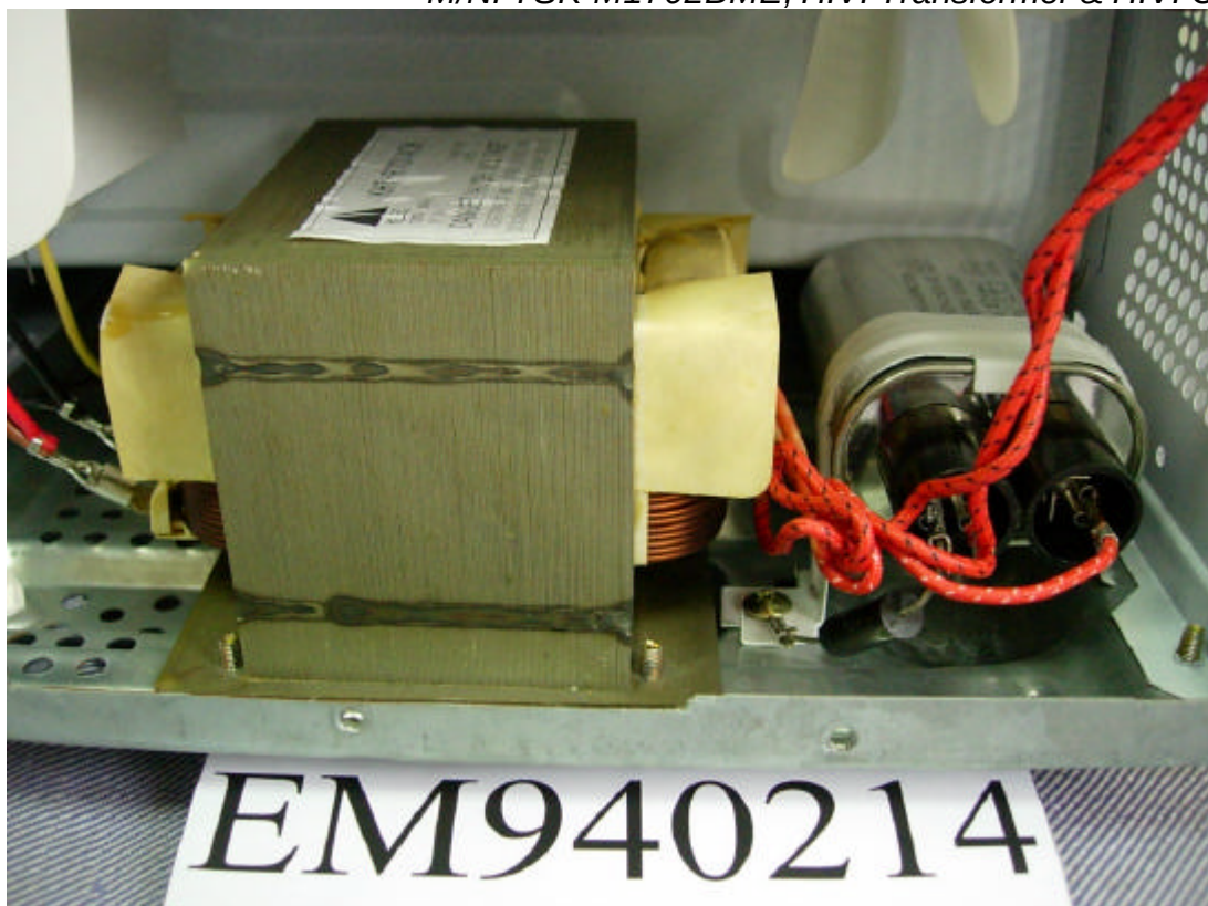
Photo 18 M/N: TSK-M1702BME, H.V. Transformer & H.V. Capacitor
