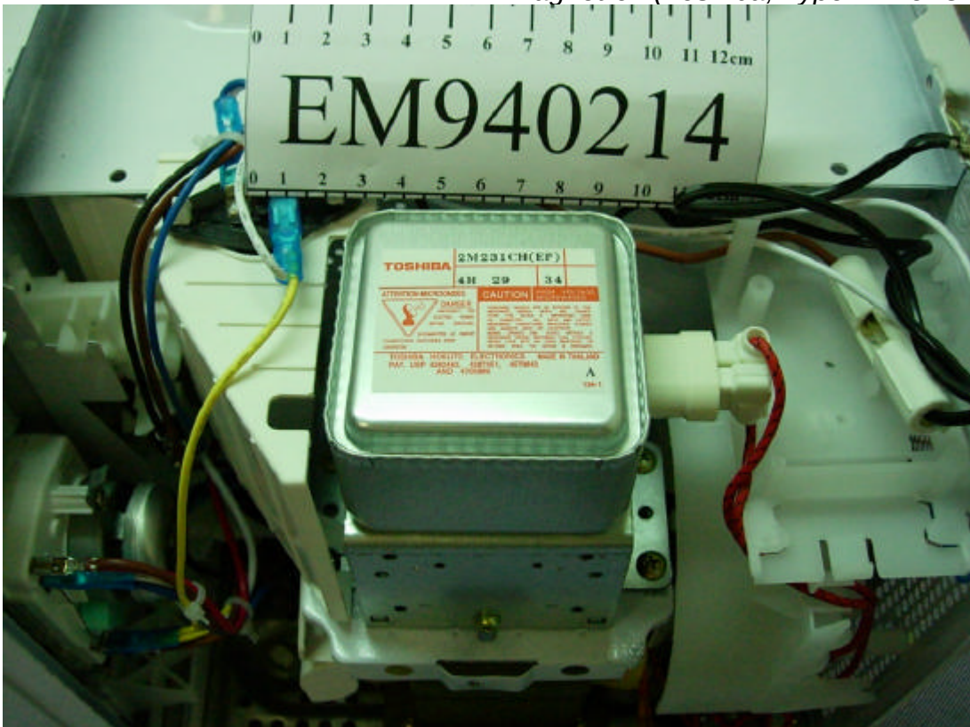
Photo 44 Magnetron (Toshiba, Type 2M231CH(EP)-A)
