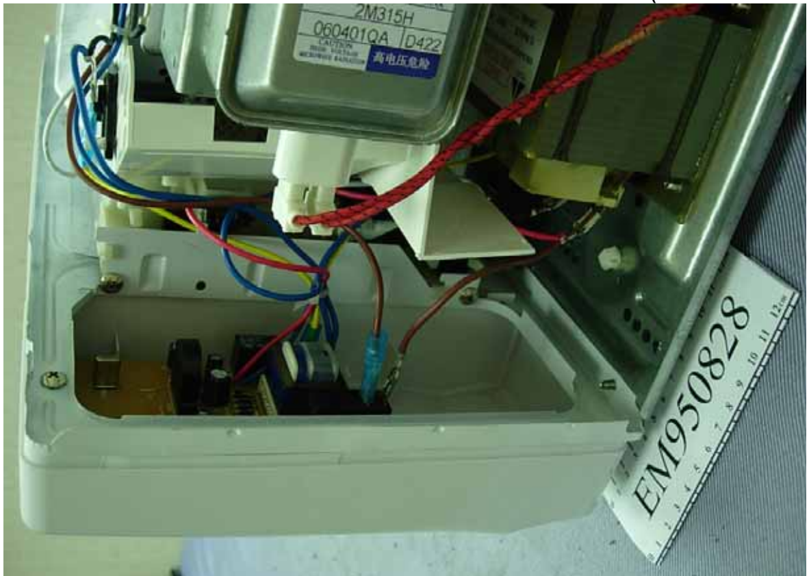
Photo 17 TSK-M1601ME Internal View (Removed the Control Panel Cover)
