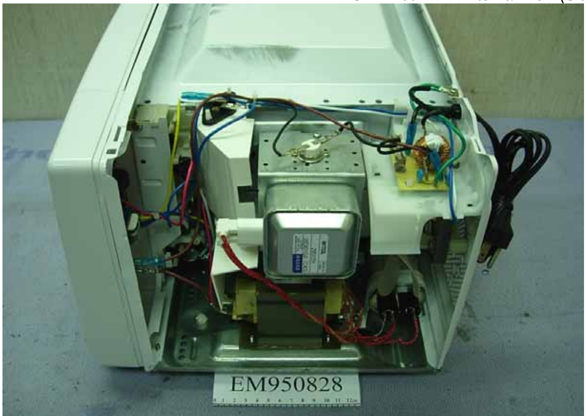
TSK-M1601ME Internal View (Side)
