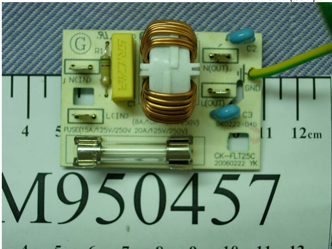
Photo 15 Filter Board (Component View)
