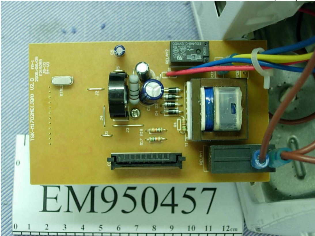
Photo 17 Main Board (Component View)
