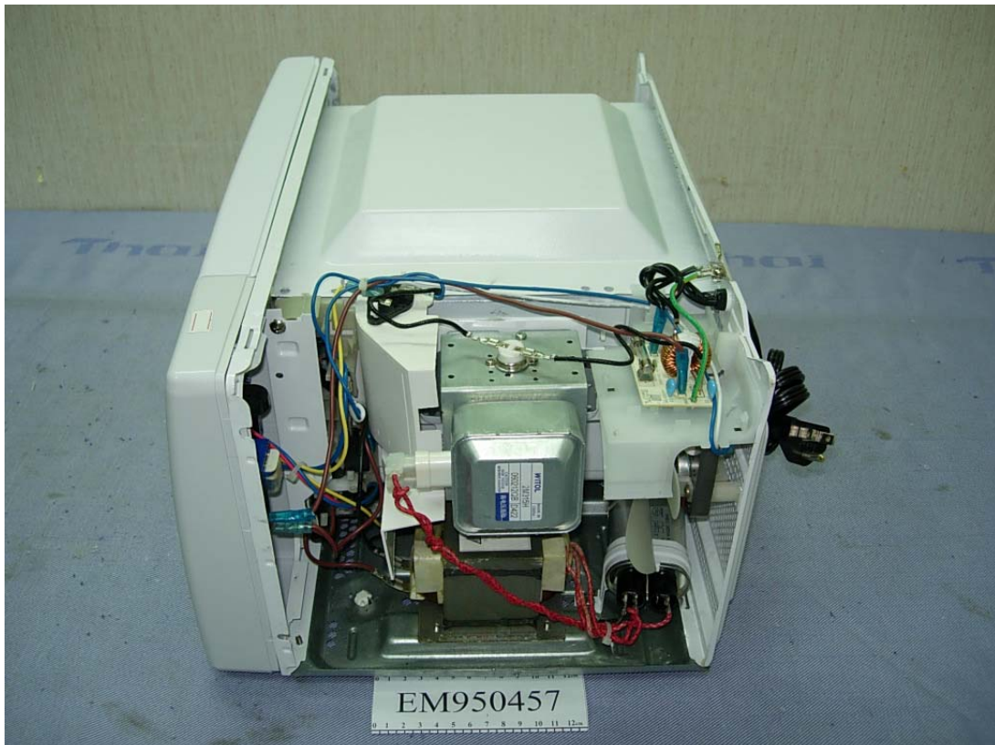
Photo 6 Internal View (Side)
