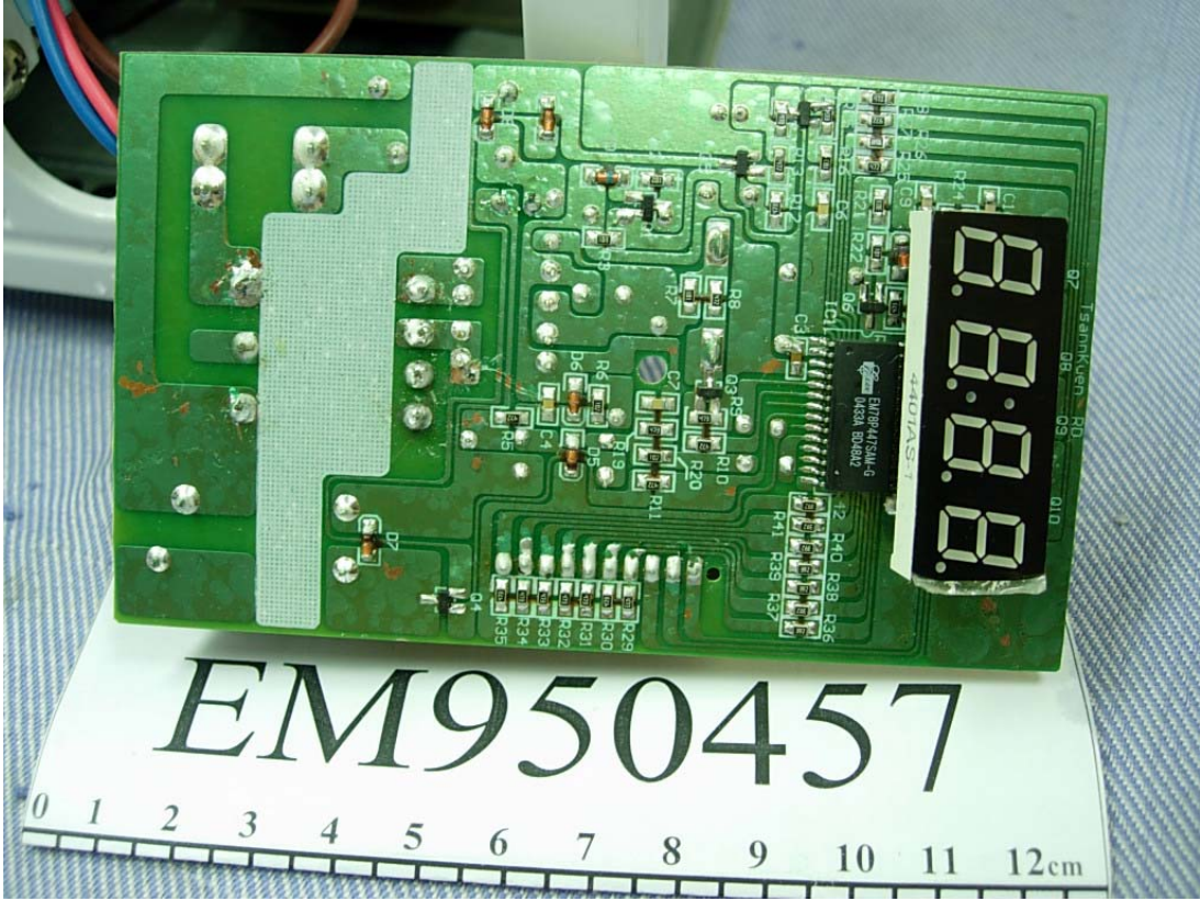
Photo 18 Main Board (Foil View)
