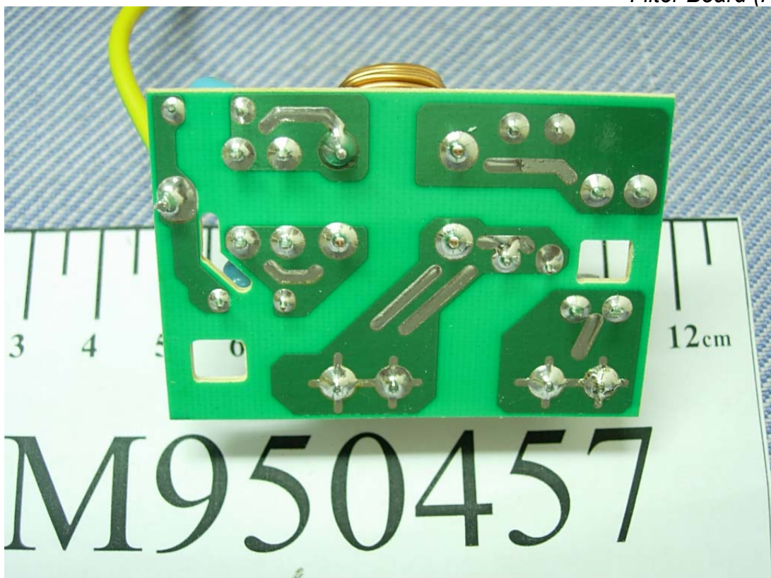
Photo 16 Filter Board (Foil View)
