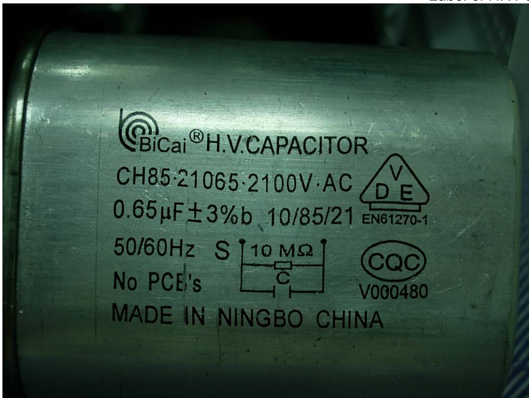
Photo 12 Label of H.V. Capacitor
