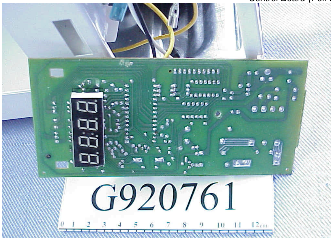
Photo 8 Control Board (Foil Side)
