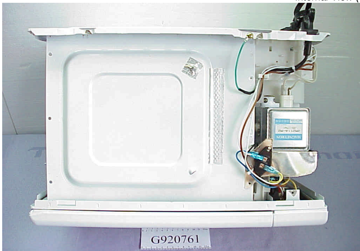
Photo 5 Internal View (Top)
