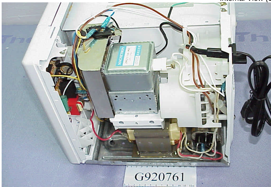
Photo 6 Internal View (Side)
