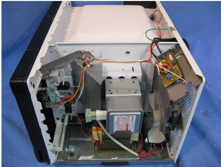
R209KK-W Internal photo
