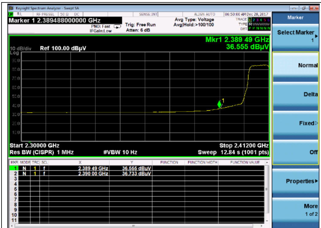
(Channel = 1 AVG, 802.11n-20)
