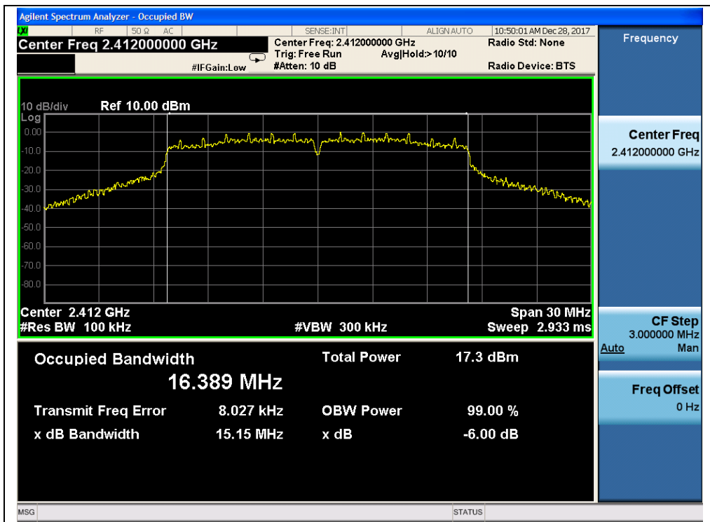
(Channel 1: 2412MHz @ 802.11g)
