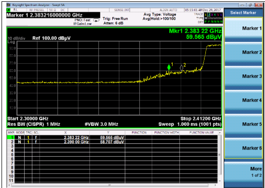
(Channel = 3 PEAK, 802.11n-40)
