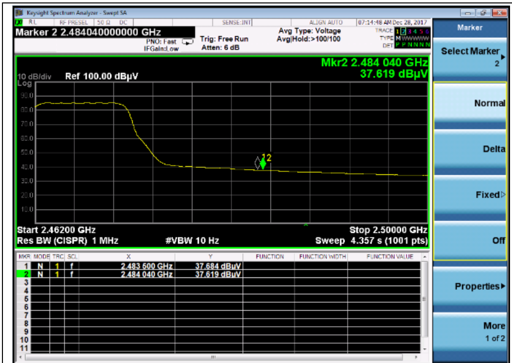
(Channel = 11 AVG, 802.11n-20)
