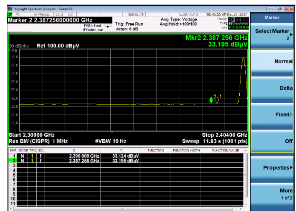
(Channel = 0, AVG)
