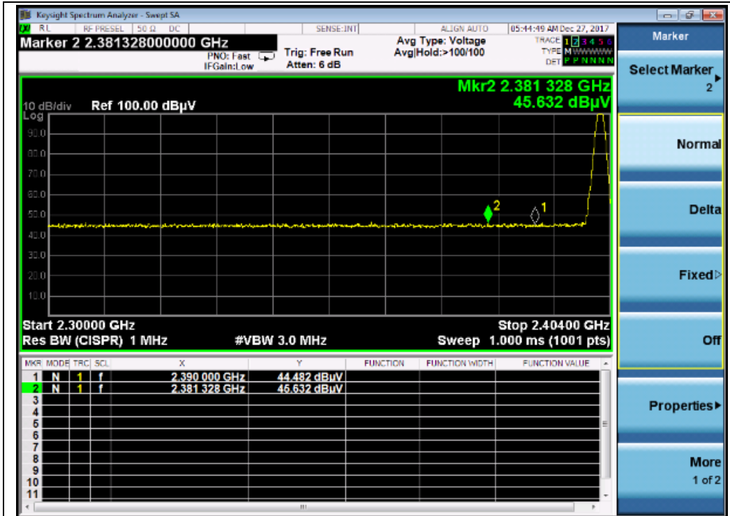
(Channel = 0, PEAK)
