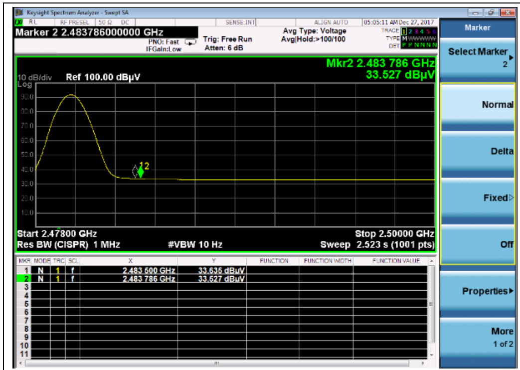
(Channel = 39, AVG)
