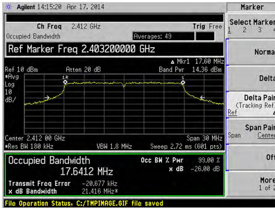
802.11 n-HT20 (Channel 1)
