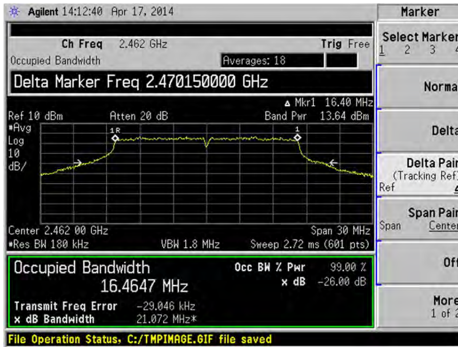
802.11 g (Channel 11)
