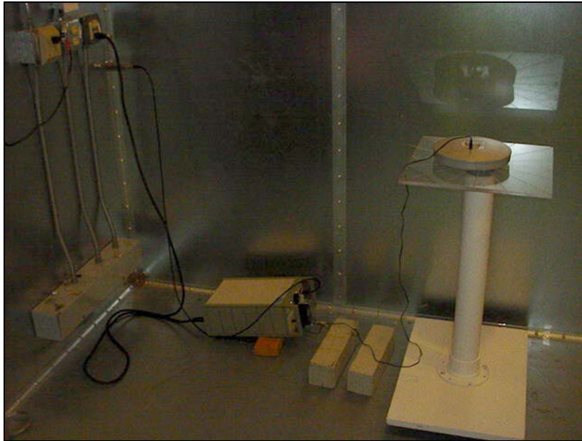
View of the EUT during Conducted Emission Testing in the 3 Meter FCC Listed Chamber
