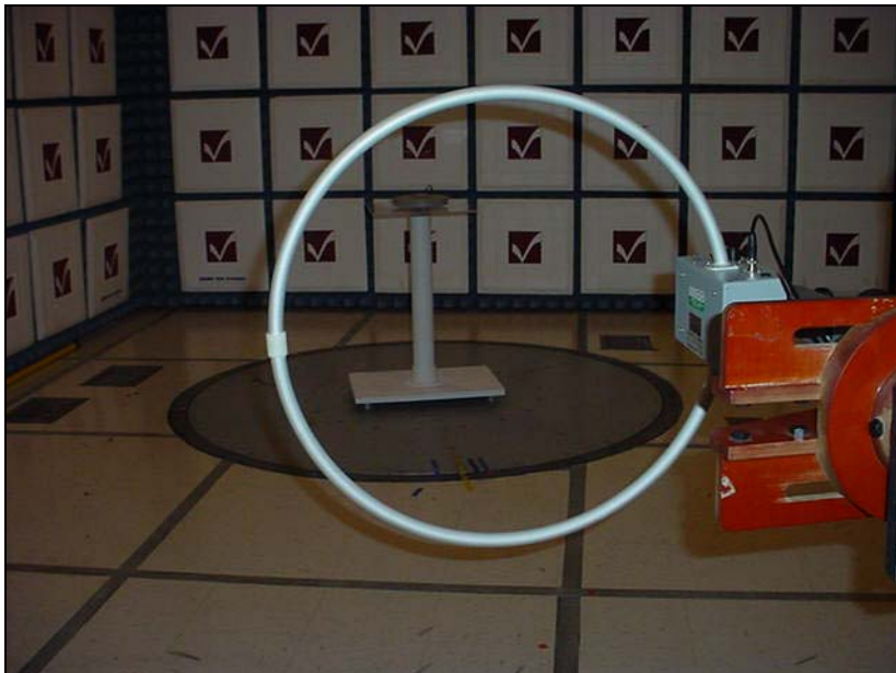
View of the EUT during Radiated Emission Investigative Testing
