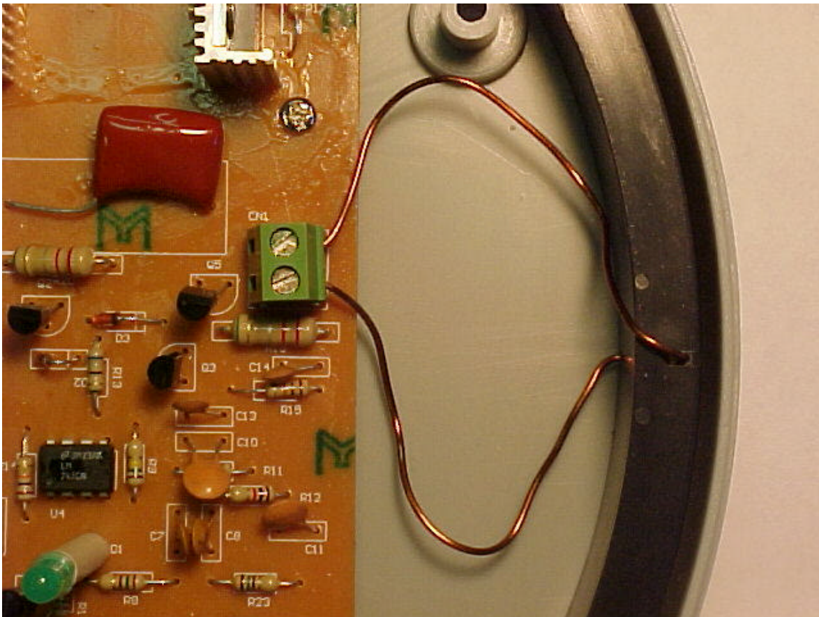
Antenna Close-up
