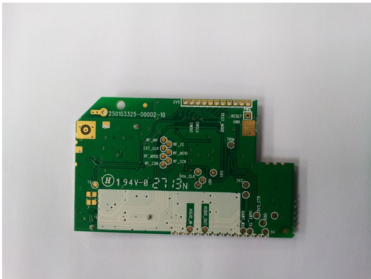
2.4 GHz MODULE PCB BOTTOM VIEW
