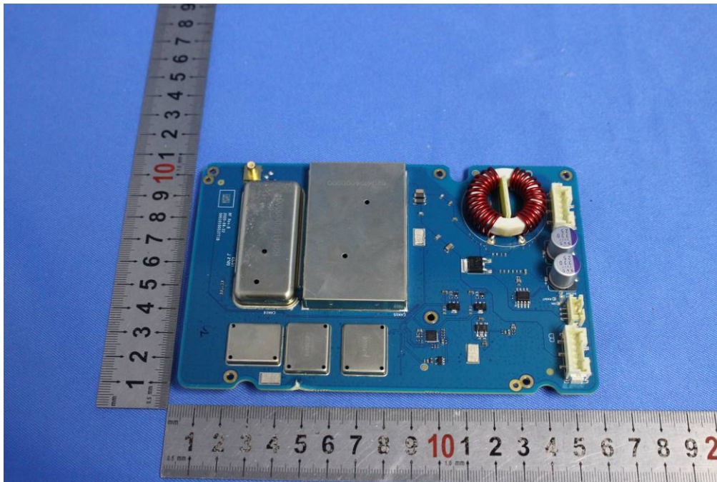
VHF/DSC Board
