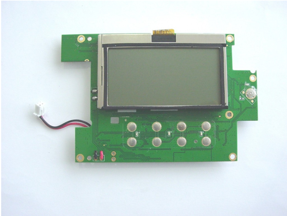
CPU PCB – TOP VIEW
