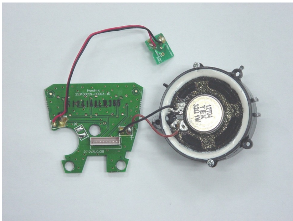
HANDMIC PCB – BOTTOM VIEW
