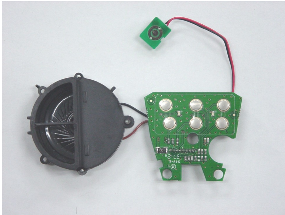
HANDMIC PCB – TOP VIEW
