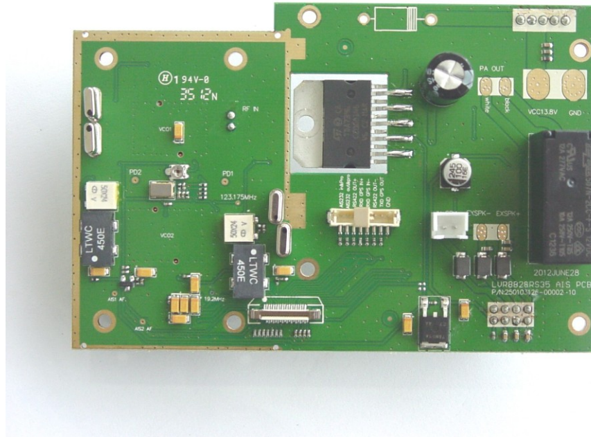
AIS PCB – BOTTOM VIEW
