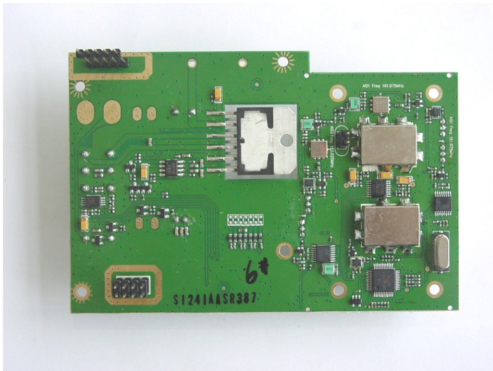
AIS PCB – BOTTOM VIEW
