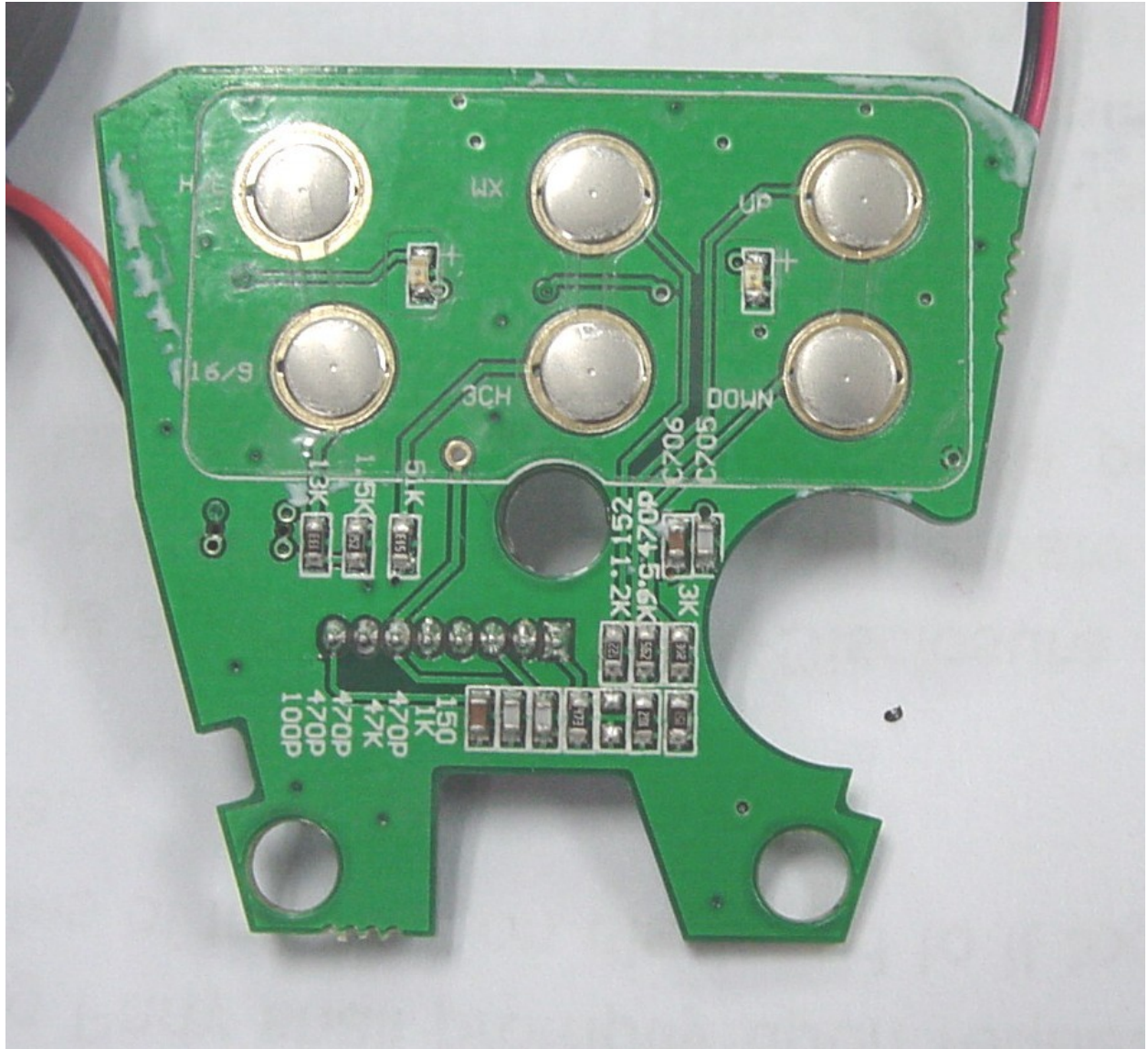
HAND MIC PCB TOP VIEW
