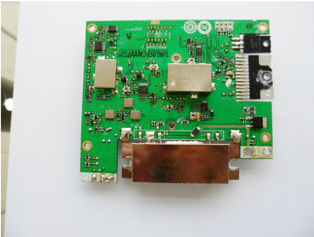
RF PCB TOP VIEW
