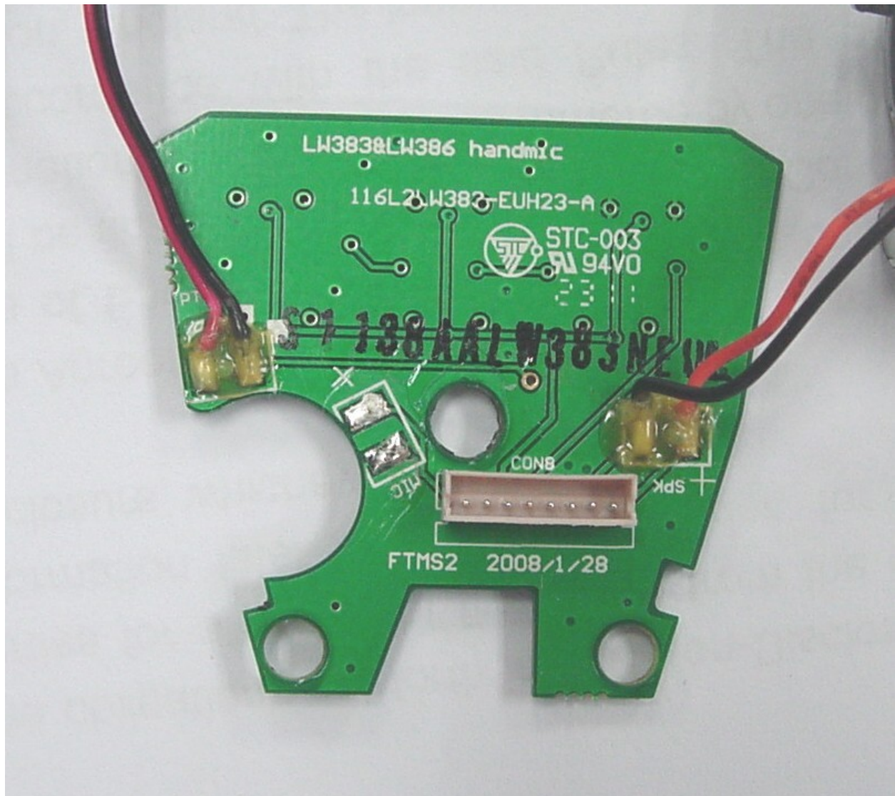
HAND MIC PCB BOTTOM VIEW
