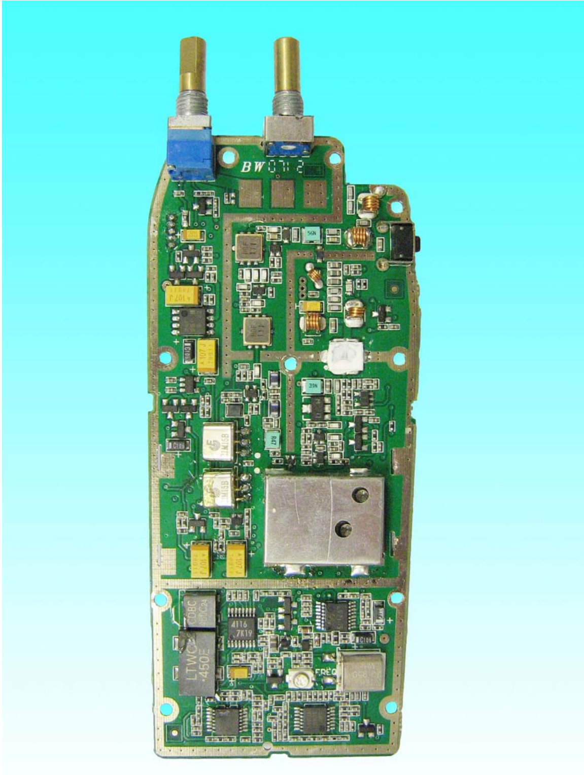
LHR20, EHR10, LHR22 Main Board with – Bottom with Shield
