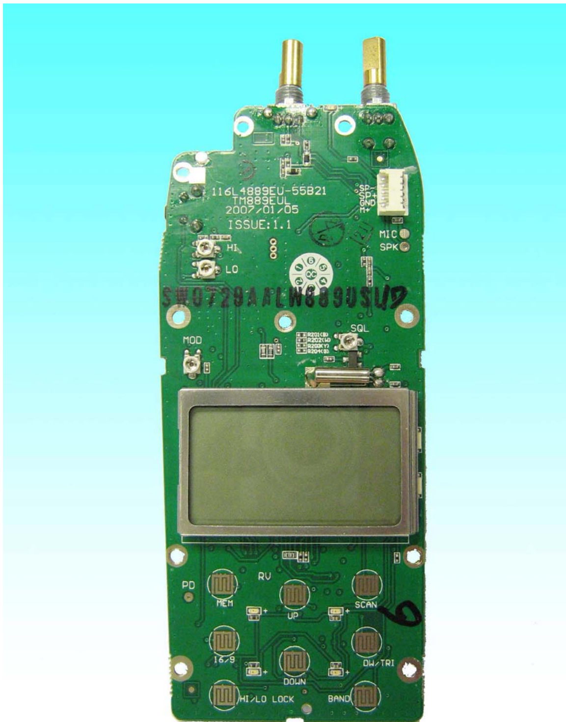
LHR20, EHR10, LHR22 Main Board – Top with Display On
