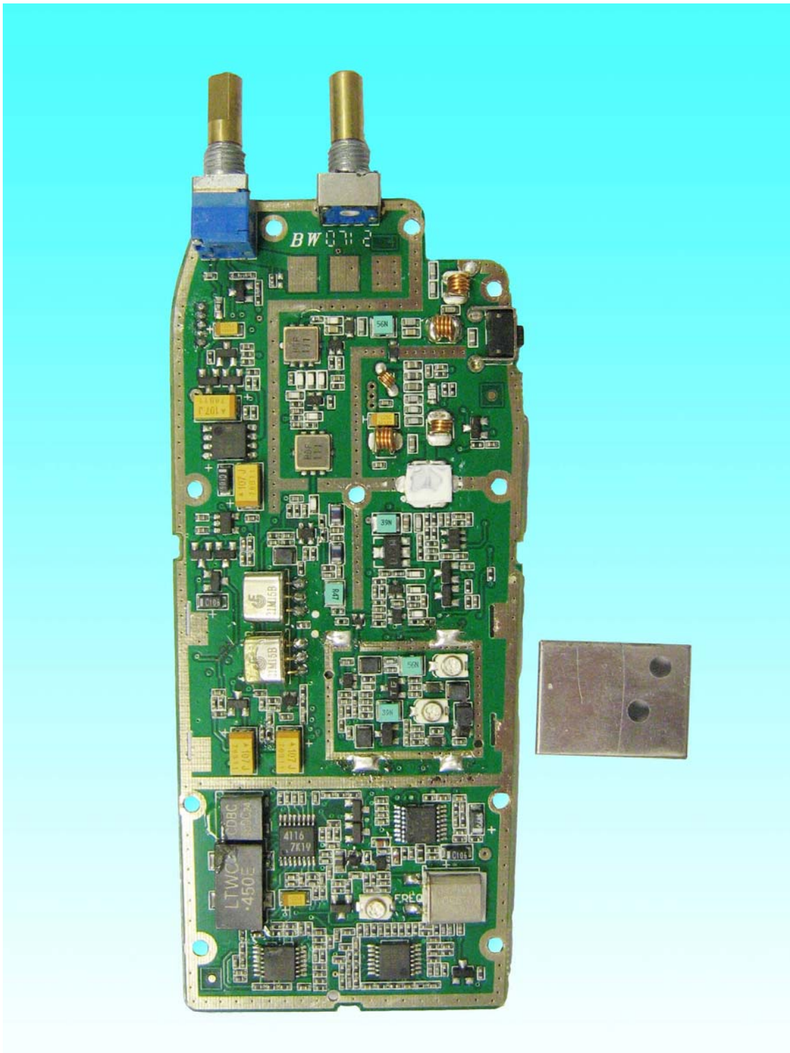
LHR20, EHR10, LHR22 Main Board with – Bottom without Shield
