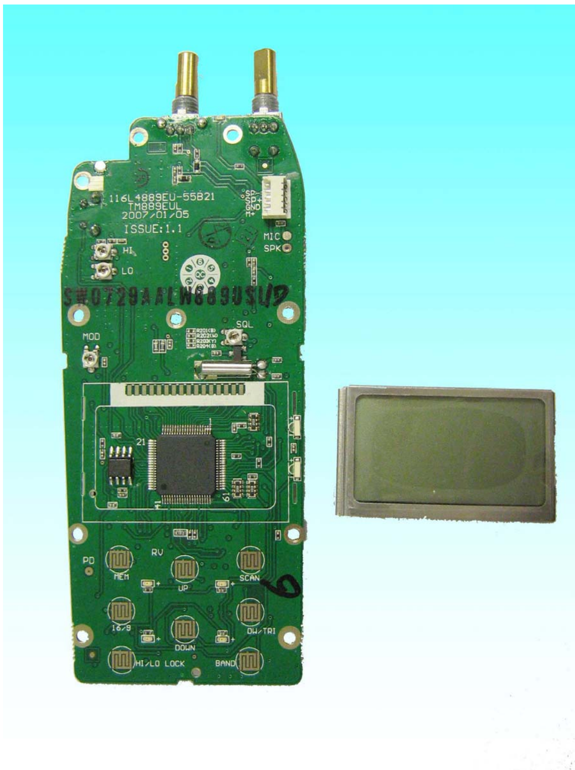
LHR20, EHR10, LHR22 Main Board – Top with Display Removed
