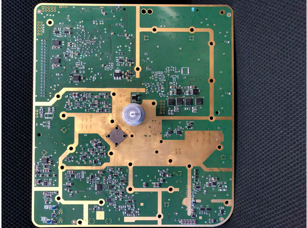
RF PCB
