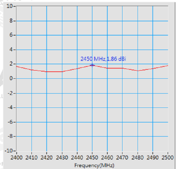
Maximum Peak Gain at 2450MHz : 1.86dBi
