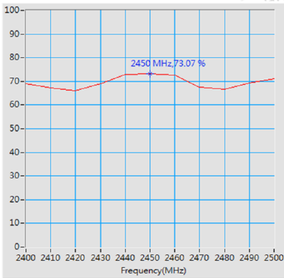
Maximum Efficiency at 2450MHz : 73.07%
