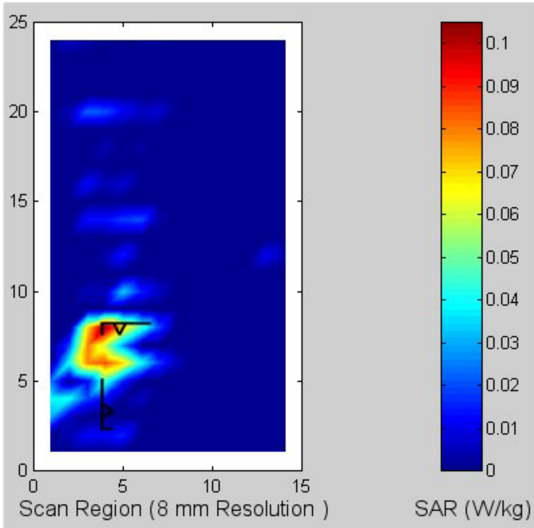
Fig. F.1. Above-lap position (Configuration 1). Normal mode at 5.26 GHz. Coarse scan for the highest SAR region for the Arcadyan EZ-Stream Universal Wireless Cardbus Adapter inserted into Dell Model PP01L Host Computer.
