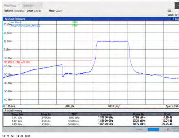
Band25-1.4MHz-QPSK-26047-6RB#0
