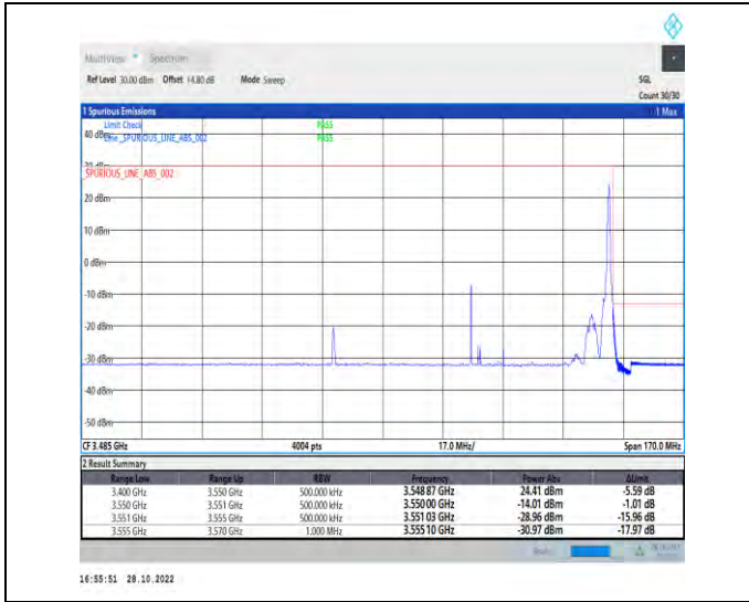
1-N77-3450-3550-PC2-30-80-H-2-DFT-PI2BPSK-Edge_1RB_Right-1@216-Ant1-1--PASS-see graph
