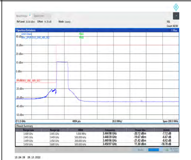
1-N77-3450-3550-PC2-30-15-L-6-CP-QPSK-Outer_Full-38@0-Ant1-1--PASS-see graph
