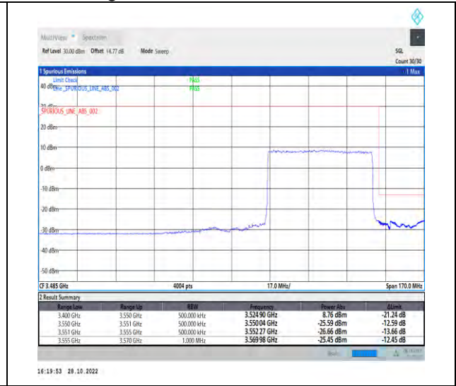
1-N77-3450-3550-PC2-30-50-H-3-DFT-PI2BPSK-Outer_Full-128@0-Ant1-1--PASS-see graph
