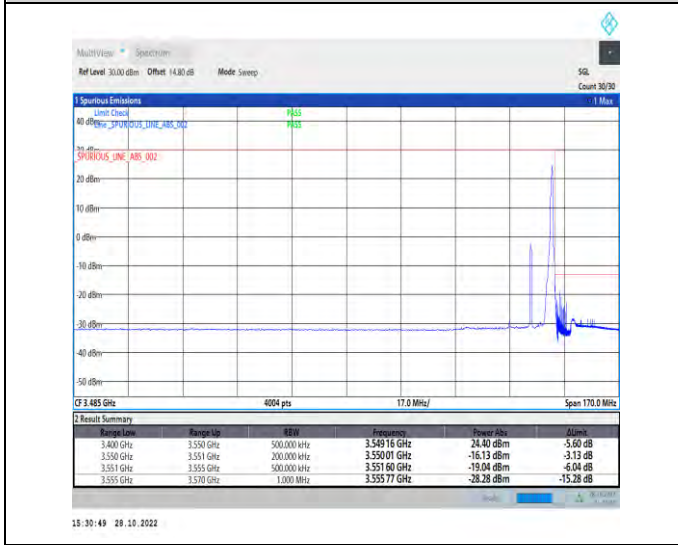
1-N77-3450-3550-PC2-30-15-H-5-CP-QPSK-Edge_1RB_Right-1@37-Ant1-1--PASS-see graph
