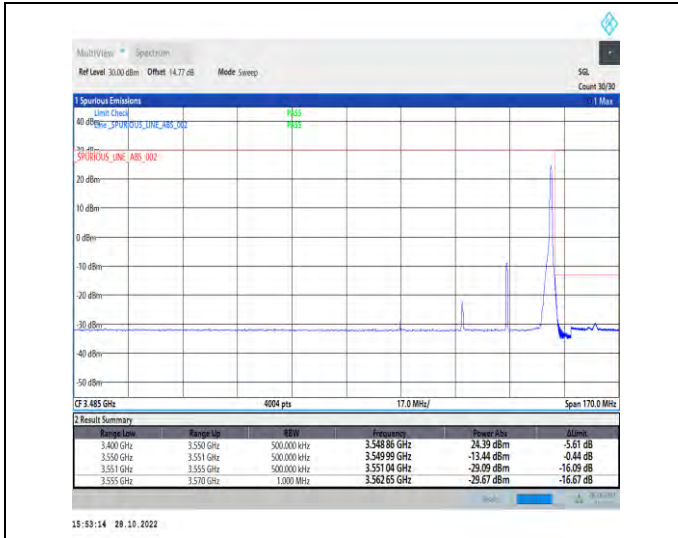
1-N77-3450-3550-PC2-30-30-H-2-DFT-PI2BPSK-Edge_1RB_Right-1@77-Ant1-1--PASS-see graph
