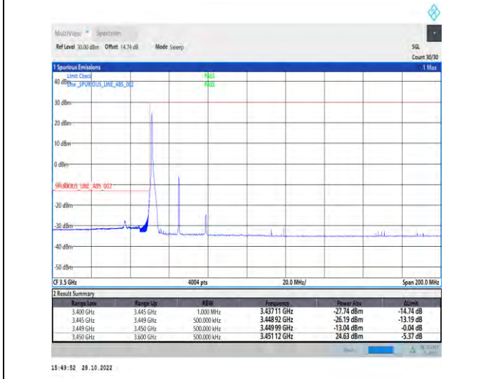
1-N77-3450-3550-PC2-30-30-L-4-CP-QPSK-Edge_1RB_Left-1@0-Ant1-1--PASS-see graph
