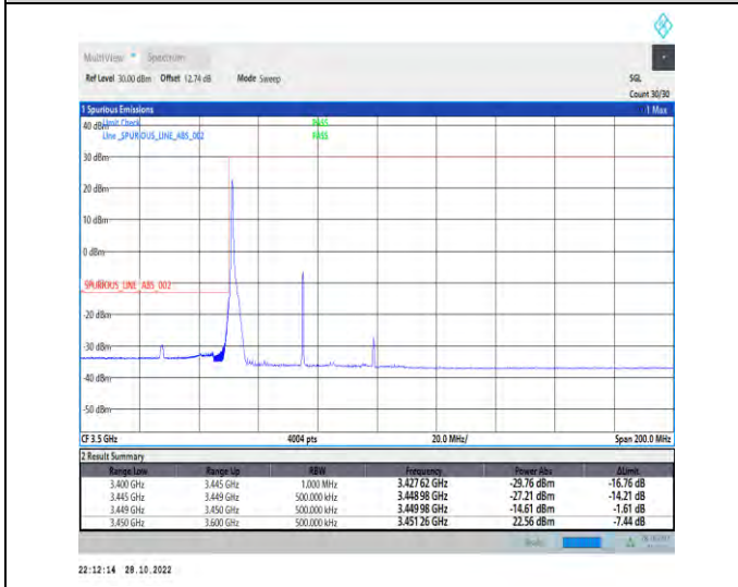
1-N77-3450-3550-PC2-30-50-L-4-CP-QPSK-Edge_1RB_Left-1@0-Ant1-1--PASS-see graph
