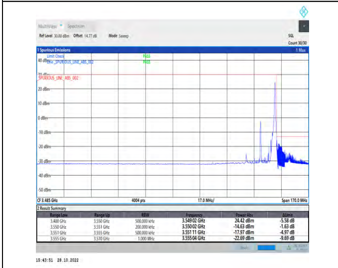
1-N77-3450-3550-PC2-30-20-H-5-CP-QPSK-Edge_1RB_Right-1@50-Ant1-1--PASS-see graph
