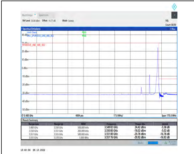
1-N77-3450-3550-PC2-30-20-H-2-DFT-PI2BPSK-Edge_1RB_Right-1@50-Ant1-1--PASS-see graph
