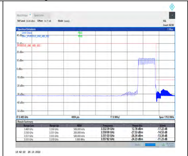
1-N77-3450-3550-PC2-30-20-H-3-DFT-PI2BPSK-Outer_Full-50@0-Ant1-1--PASS-see graph
