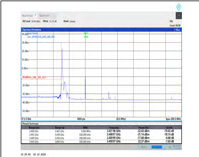
1-N77-3450-3550-PC2-30-60-L-1-DFT-PI2BPSK-Edge_1RB_Left-1@0-Ant1-1--PASS-see graph
