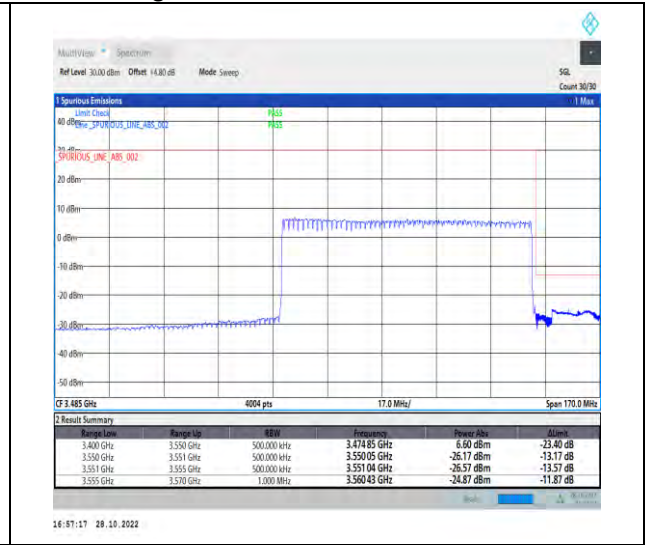
1-N77-3450-3550-PC2-30-80-H-3-DFT-PI2BPSK-Outer_Full-216@0-Ant1-1--PASS-see graph
