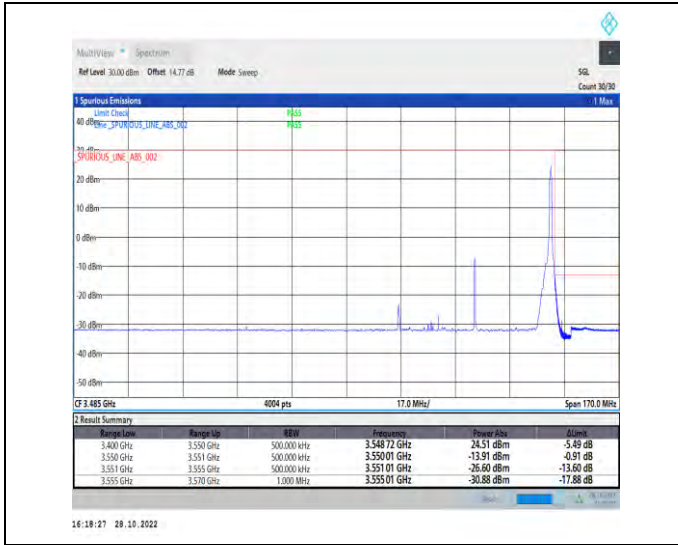
1-N77-3450-3550-PC2-30-50-H-2-DFT-PI2BPSK-Edge_1RB_Right-1@132-Ant1-1--PASS-see graph
