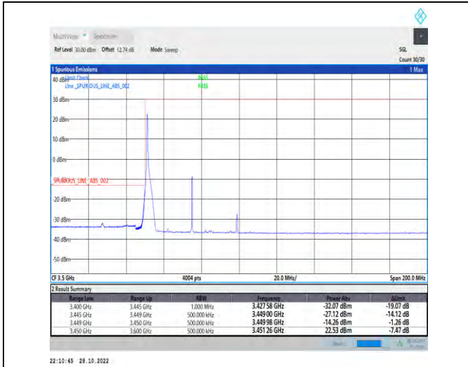
1-N77-3450-3550-PC2-30-50-L-1-DFT-PI2BPSK-Edge_1RB_Left-1@0-Ant1-1--PASS-see graph
