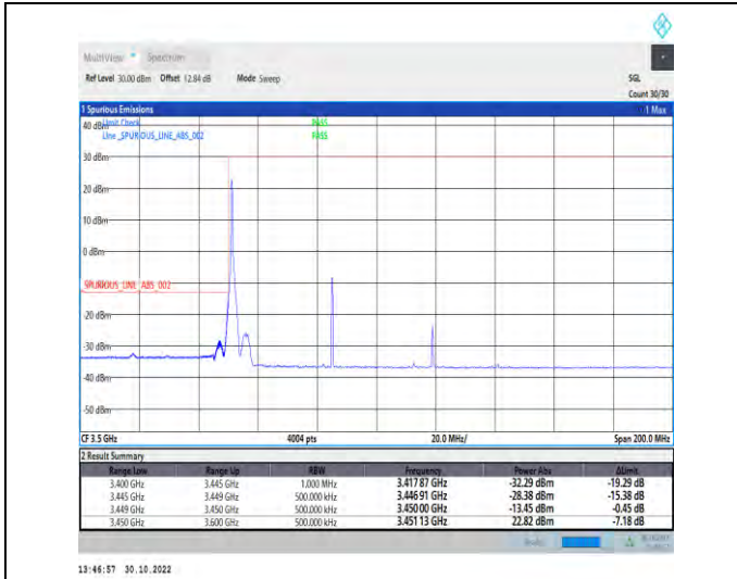
1-N77-3450-3550-PC2-30-70-L-1-DFT-PI2BPSK-Edge_1RB_Left-1@0-Ant1-1--PASS-see graph
