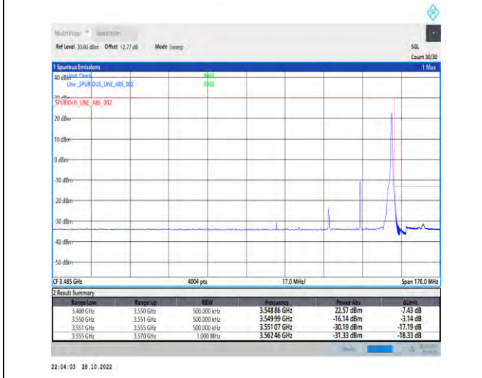
1-N77-3450-3550-PC2-30-30-H-5-CP-QPSK-Edge_1RB_Right-1@77-Ant1-1--PASS-see graph
