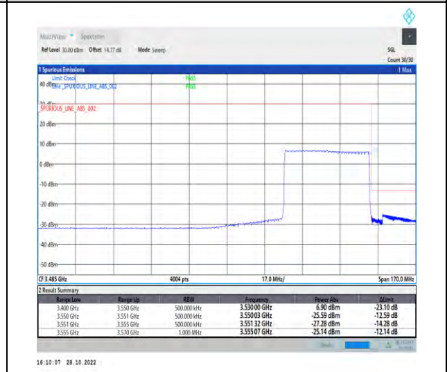
1-N77-3450-3550-PC2-30-40-H-6-CP-QPSK-Outer_Full-106@0-Ant1-1--PASS-see graph
