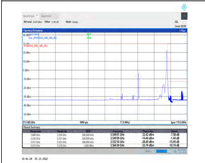
1-N77-3450-3550-PC2-30-60-H-5-CP-QPSK-Edge_1RB_Right-1@161-Ant1-1--PASS-see graph
