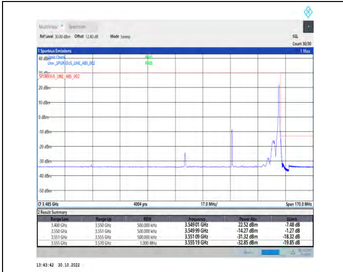
1-N77-3450-3550-PC2-30-60-H-2-DFT-PI2BPSK-Edge_1RB_Right-1@161-Ant1-1--PASS-see graph
