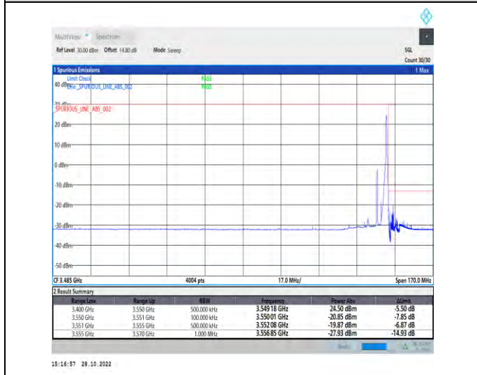
1-N77-3450-3550-PC2-30-10-H-5-CP-QPSK-Edge_1RB_Right-1@23-Ant1-1--PASS-see graph
