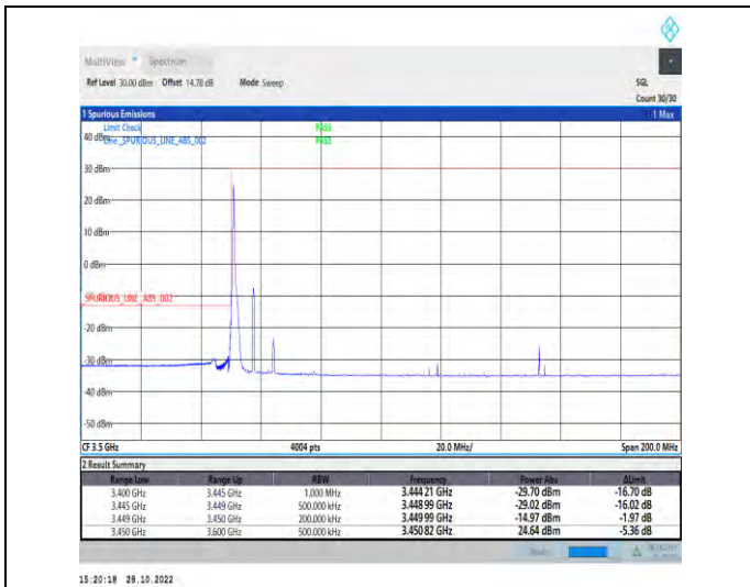
1-N77-3450-3550-PC2-30-15-L-1-DFT-PI2BPSK-Edge_1RB_Left-1@0-Ant1-1--PASS-see graph
