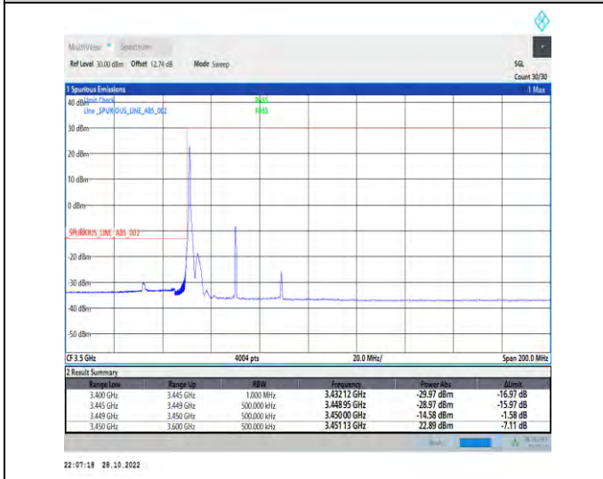
1-N77-3450-3550-PC2-30-40-L-4-CP-QPSK-Edge_1RB_Left-1@0-Ant1-1--PASS-see graph
