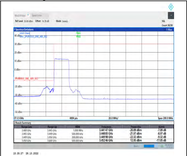
1-N77-3450-3550-PC2-30-20-L-3-DFT-PI2BPSK-Outer_Full-50@0-Ant1-1--PASS-see graph
