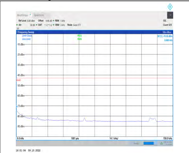
1-N77-3700-3980-PC2-30-100-L-1-DFT-QPSK-Edge _1RB_Left-1@0-0.009-0.15-Ant1-0.01--74.35--43-PA SS
