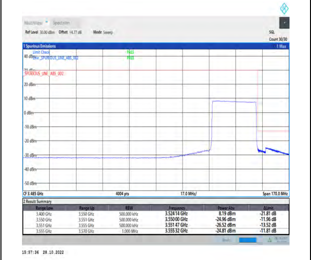
1-N77-3450-3550-PC2-30-30-H-6-CP-QPSK-Outer_Full-78@0-Ant1-1--PASS-see graph
