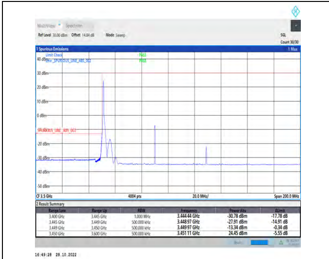
1-N77-3450-3550-PC2-30-80-L-1-DFT-PI2BPSK-Edge_1RB_Left-1@0-Ant1-1--PASS-see graph
