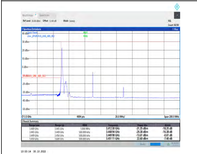
1-N77-3450-3550-PC2-30-80-L-4-CP-QPSK-Edge_1RB_Left-1@0-Ant1-1--PASS-see graph
