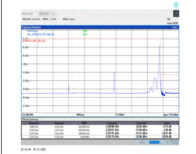
1-N77-3450-3550-PC2-30-100-H-5-CP-QPSK-Edge_1RB_Right-1@272-Ant1-1--PASS-see graph
