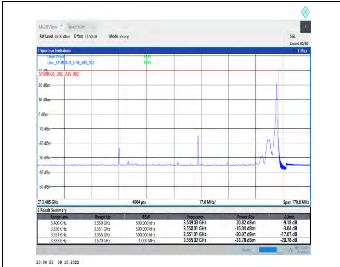
1-N77-3450-3550-PC2-30-100-H-2-DFT-QPSK-Edge_1RB_Right-1@272-Ant1-1--PASS-see graph
