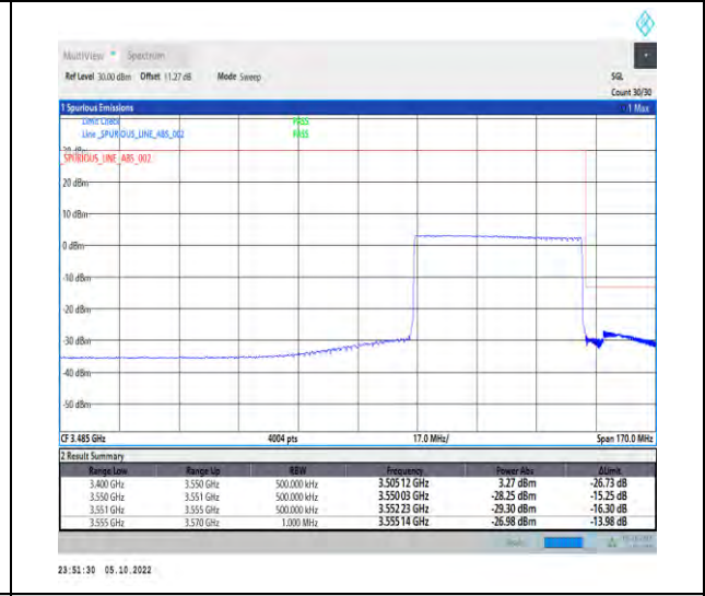
1-N77-3450-3550-PC2-30-50-H-6-CP-QPSK-Outer_Full-133@0-Ant1-1--PASS-see graph
