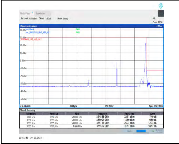
1-N77-3450-3550-PC2-30-70-H-5-CP-QPSK-Edge_1RB_Right-1@188-Ant1-1--PASS-see graph
