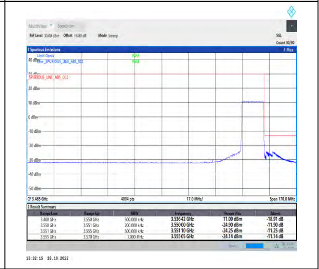
1-N77-3450-3550-PC2-30-15-H-6-CP-QPSK-Outer_Full-38@0-Ant1-1--PASS-see graph
