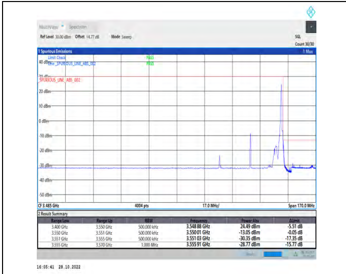
1-N77-3450-3550-PC2-30-40-H-2-DFT-PI2BPSK-Edge_1RB_Right-1@105-Ant1-1--PASS-see graph
