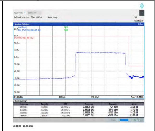
1-N77-3450-3550-PC2-30-70-H-3-DFT-PI2BPSK-Outer_Full-180@0-Ant1-1--PASS-see graph
