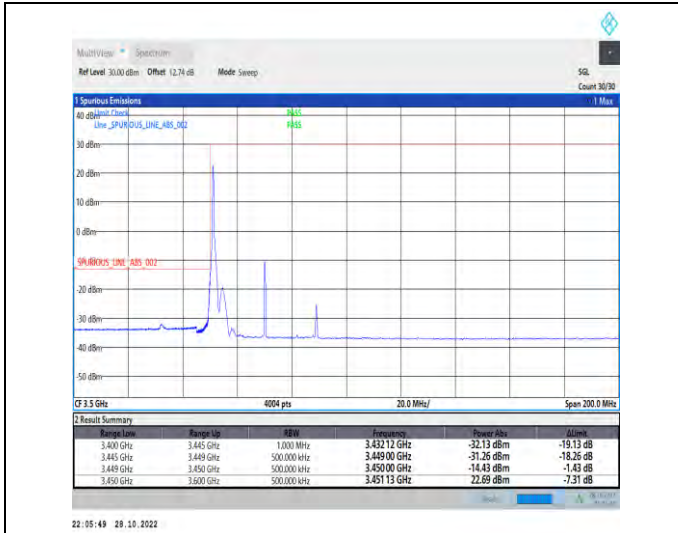
1-N77-3450-3550-PC2-30-40-L-1-DFT-PI2BPSK-Edge_1RB_Left-1@0-Ant1-1--PASS-see graph
