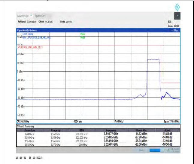
1-N77-3450-3550-PC2-30-15-H-3-DFT-PI2BPSK-Outer_Full-36@0-Ant1-1--PASS-see graph
