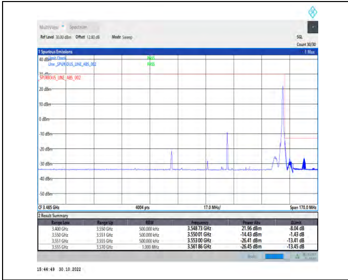
1-N77-3450-3550-PC2-30-70-H-2-DFT-PI2BPSK-Edge_1RB_Right-1@188-Ant1-1--PASS-see graph
