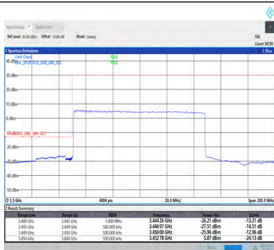
1-N77-3450-3550-PC2-30-100-L-3-DFT-PI2B PSK-Outer_Full-270@0-Ant1-1--PASS-see graph
