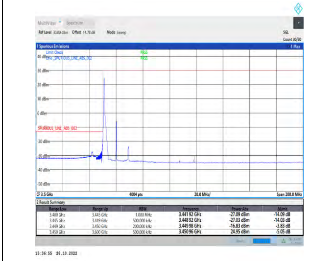
1-N77-3450-3550-PC2-30-20-L-4-CP-QPSK-Edge_1RB_Left-1@0-Ant1-1--PASS-see graph
