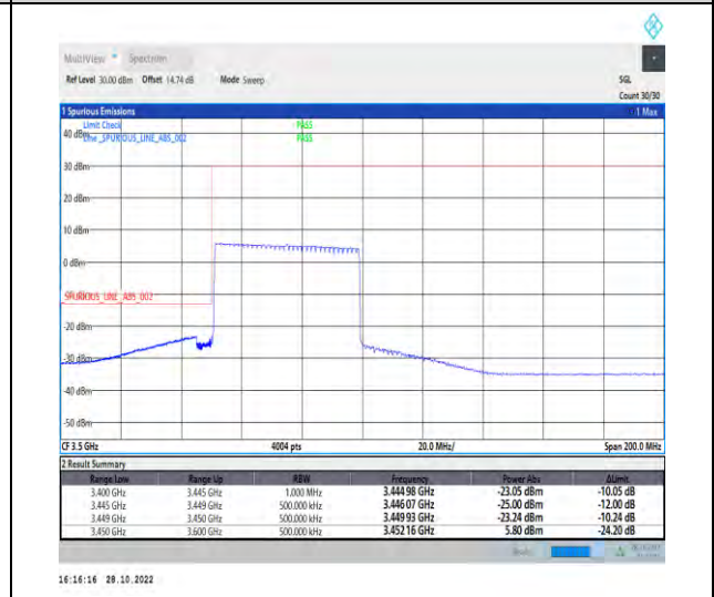
1-N77-3450-3550-PC2-30-50-L-6-CP-QPSK-Outer_Full-133@0-Ant1-1--PASS-see graph
