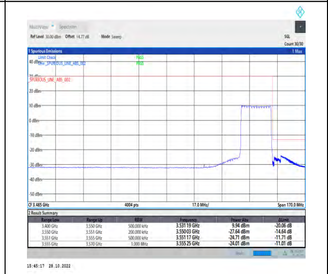
1-N77-3450-3550-PC2-30-20-H-6-CP-QPSK-Outer_Full-51@0-Ant1-1--PASS-see graph
