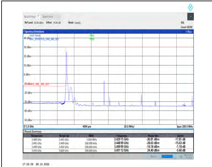
1-N77-3450-3550-PC2-30-90-L-1-DFT-PI2BPSK-Edge_1RB_Left-1@0-Ant1-1--PASS-see graph
