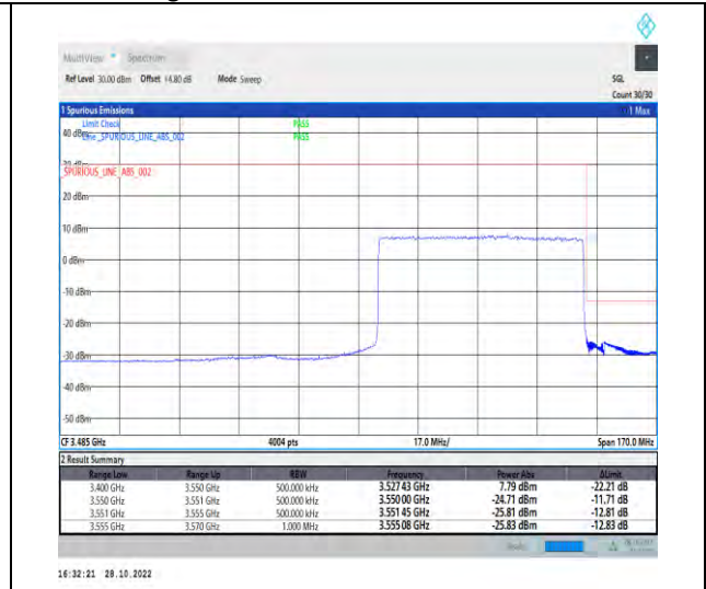
1-N77-3450-3550-PC2-30-60-H-3-DFT-PI2BPSK-Outer_Full-162@0-Ant1-1--PASS-see graph
