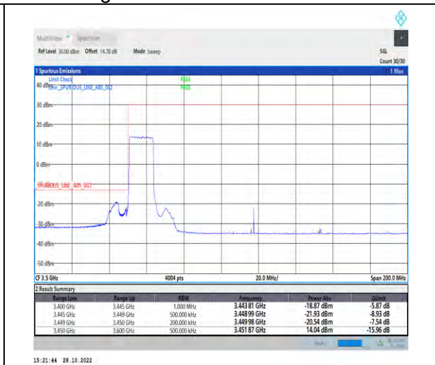
1-N77-3450-3550-PC2-30-15-L-3-DFT-PI2BPSK-Outer_Full-36@0-Ant1-1--PASS-see graph
