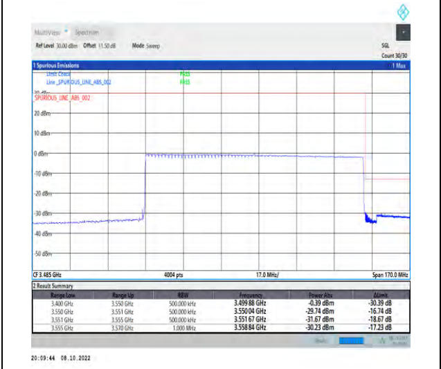
1-N77-3450-3550-PC2-30-100-H-6-CP-QPSK-Outer_Full-273@0-Ant1-1--PASS-see graph
