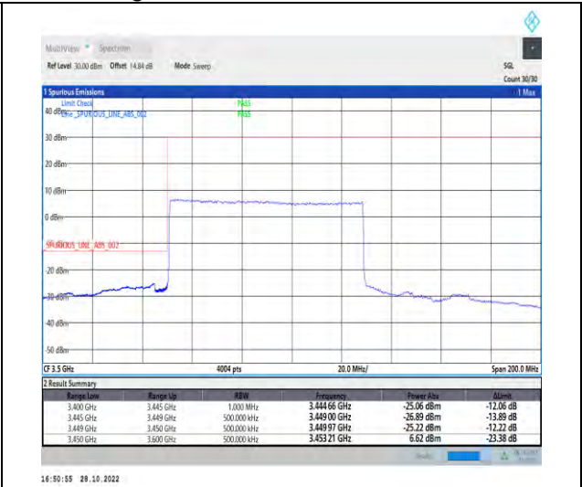
1-N77-3450-3550-PC2-30-80-L-3-DFT-PI2BPSK-Outer_Full-216@0-Ant1-1--PASS-see graph
