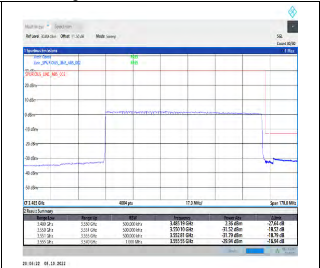
1-N77-3450-3550-PC2-30-100-H-3-DFT-QPSK-Outer_Full-270@0-Ant1-1--PASS-see graph
