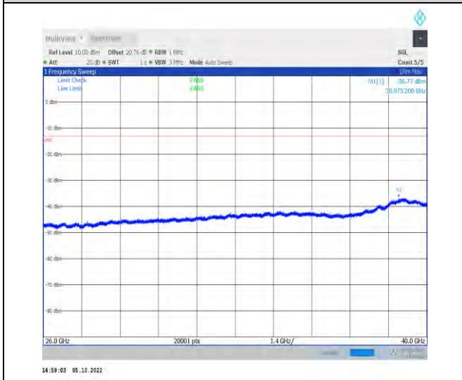
1-N77-3450-3550-PC2-30-100-L-1-DFT-QPSK-Edge _1RB_Left-1@0-26000-40000-Ant1-26000.00--42.39 --13-PASS
