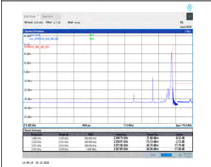
1-N77-3450-3550-PC2-30-40-H-5-CP-QPSK-Edge_1RB_Right-1@105-Ant1-1--PASS-see graph
