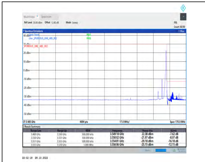
1-N77-3450-3550-PC2-30-10-H-2-DFT-PI2BPSK-Edge_1RB_Right-1@23-Ant1-1--PASS-see graph
