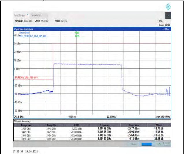
1-N77-3450-3550-PC2-30-90-L-3-DFT-PI2BPSK-Outer_Full-240@0-Ant1-1--PASS-see graph
