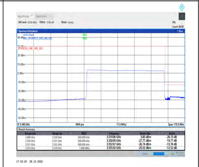
1-N77-3450-3550-PC2-30-80-H-6-CP-QPSK-Outer_Full-217@0-Ant1-1--PASS-see graph
