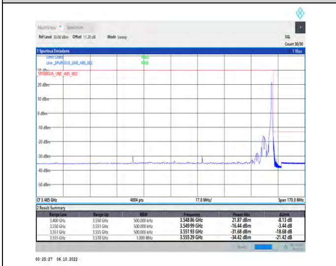
1-N77-3450-3550-PC2-30-90-H-5-DFT-PI2BPSK-Edge_1RB_Right-1@244-Ant1-1--PASS-see graph
