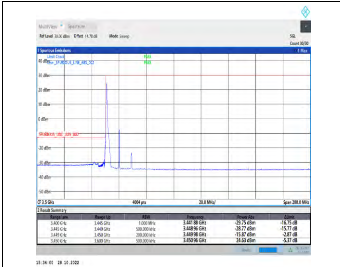
1-N77-3450-3550-PC2-30-20-L-1-DFT-PI2BPSK-Edge_1RB_Left-1@0-Ant1-1--PASS-see graph
