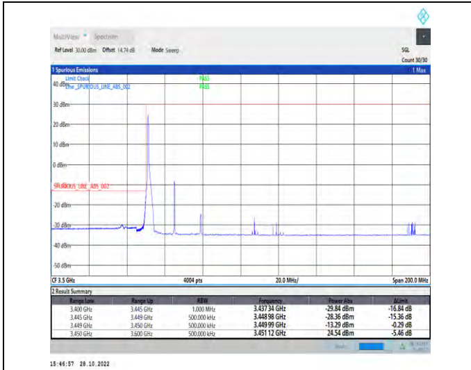
1-N77-3450-3550-PC2-30-30-L-1-DFT-PI2BPSK-Edge_1RB_Left-1@0-Ant1-1--PASS-see graph
