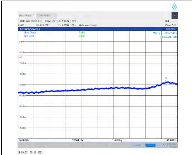
1-N77-3450-3550-PC2-30-100-H-1-DFT-QPSK-Edge _1RB_Left-1@0-26000-40000-Ant1-26000.00--42.46 --13-PASS
