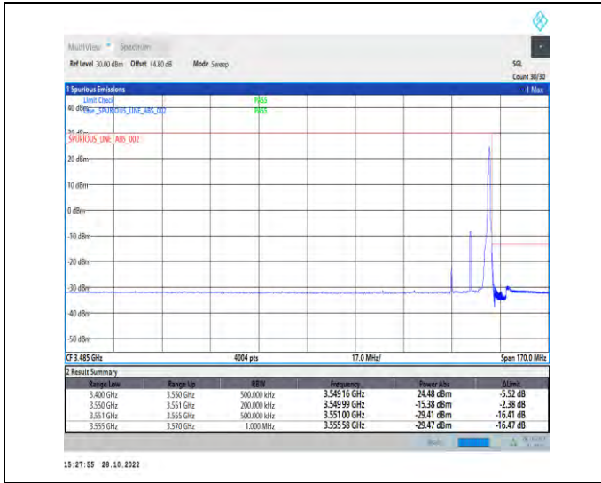
1-N77-3450-3550-PC2-30-15-H-2-DFT-PI2BPSK-Edge_1RB_Right-1@37-Ant1-1--PASS-see graph
