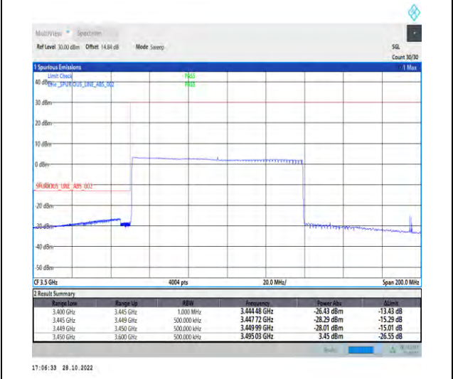
1-N77-3450-3550-PC2-30-90-L-6-CP-QPSK-Outer_Full-245@0-Ant1-1--PASS-see graph
