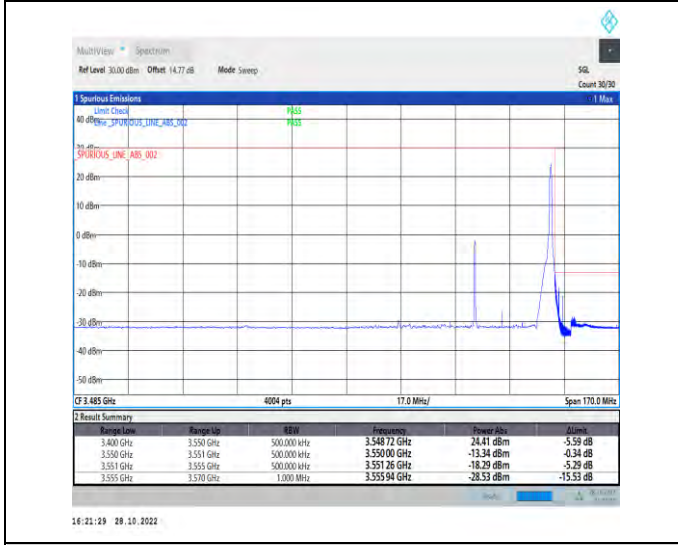
1-N77-3450-3550-PC2-30-50-H-5-CP-QPSK-Edge_1RB_Right-1@132-Ant1-1--PASS-see graph
