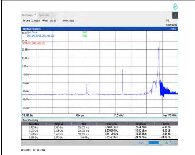
1-N77-3450-3550-PC2-30-80-H-5-CP-QPSK-Edge_1RB_Right-1@216-Ant1-1--PASS-see graph
