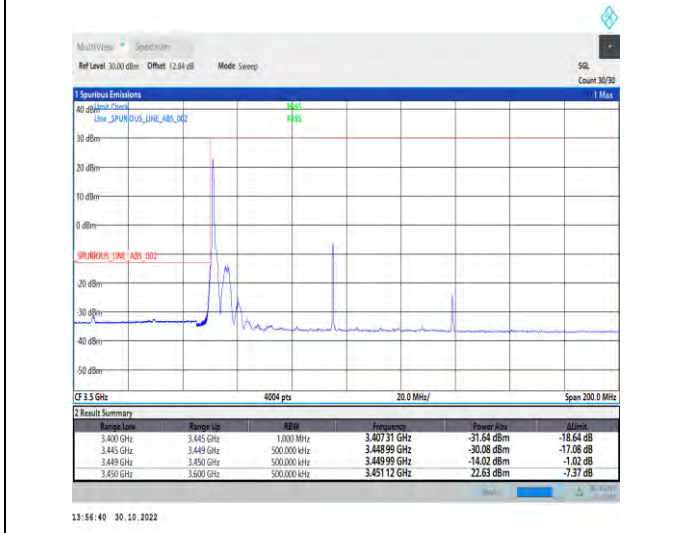
1-N77-3450-3550-PC2-30-90-L-4-CP-QPSK-Edge_1RB_Left-1@0-Ant1-1--PASS-see graph
