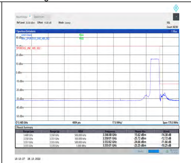
1-N77-3450-3550-PC2-30-10-H-3-DFT-PI2BPSK-Outer_Full-24@0-Ant1-1--PASS-see graph
