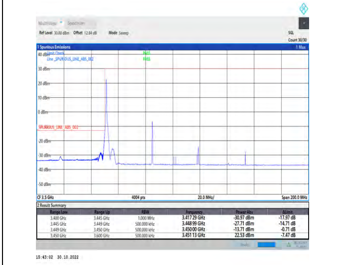
1-N77-3450-3550-PC2-30-70-L-4-CP-QPSK-Edge_1RB_Left-1@0-Ant1-1--PASS-see graph
