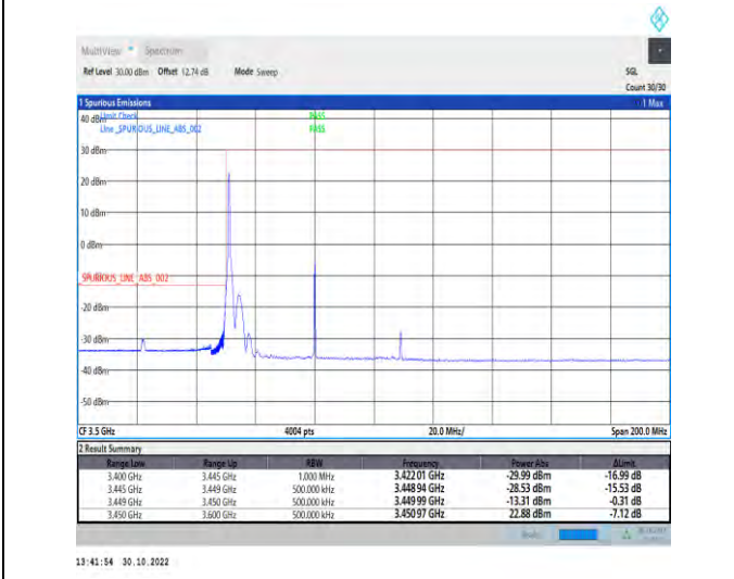
1-N77-3450-3550-PC2-30-60-L-4-CP-QPSK-Edge_1RB_Left-1@0-Ant1-1--PASS-see graph
