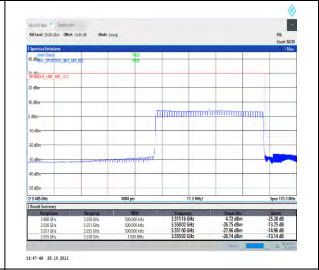
1-N77-3450-3550-PC2-30-70-H-6-CP-QPSK-Outer_Full-189@0-Ant1-1--PASS-see graph
