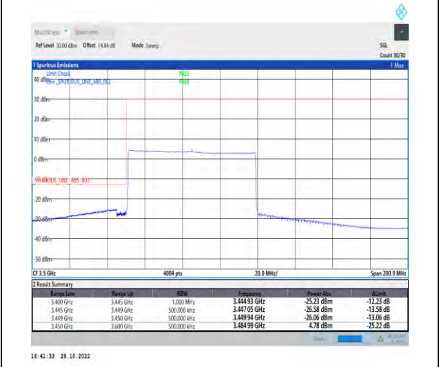
1-N77-3450-3550-PC2-30-70-L-6-CP-QPSK-Outer_Full-189@0-Ant1-1--PASS-see graph
