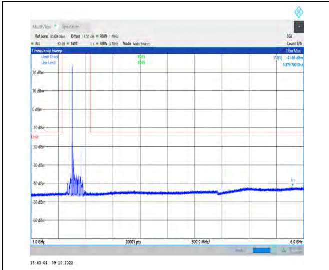
1-N77-3450-3550-PC2-30-100-L-1-DFT-QPSK-Edge _1RB_Left-1@0-3000-6000-Ant1-5879.70--41.66--1 3-PASS
