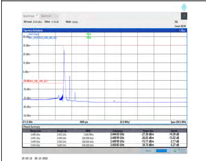
1-N77-3450-3550-PC2-30-15-L-4-CP-QPSK-Edge_1RB_Left-1@0-Ant1-1--PASS-see graph
