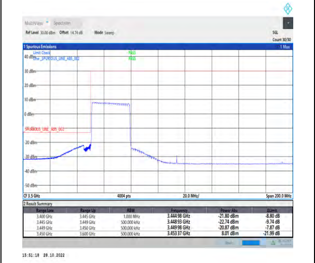
1-N77-3450-3550-PC2-30-30-L-6-CP-QPSK-Outer_Full-78@0-Ant1-1--PASS-see graph
