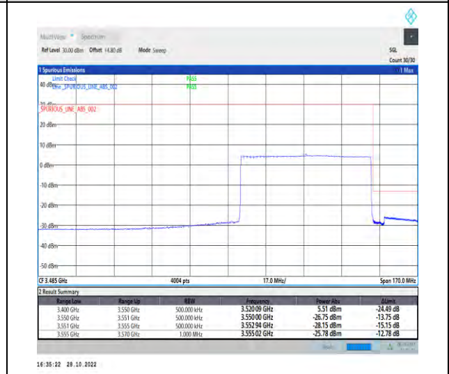
1-N77-3450-3550-PC2-30-60-H-6-CP-QPSK-Outer_Full-162@0-Ant1-1--PASS-see graph
