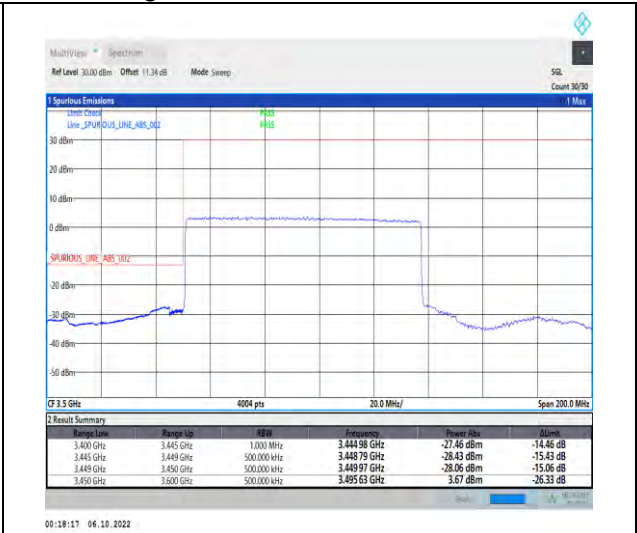
1-N77-3450-3550-PC2-30-90-L-3-DFT-QPSK-Outer_Full-240@0-Ant1-1--PASS-see graph
