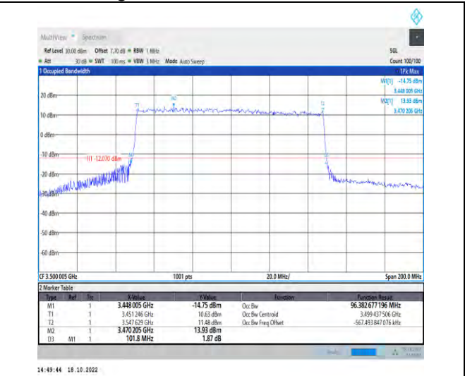
1-N77-3450-3550-PC2-30-100-M-3-DFT-16QAM-Out er_Full-270@0-Ant1-96.383-101.800-≤100-PASS
