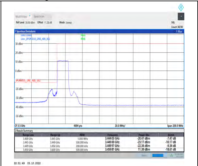
1-N77-3450-3550-PC2-30-15-L-3-DFT-QPSK-Outer_Full-36@0-Ant1-1--PASS-see graph
