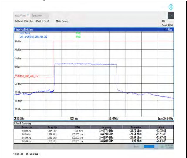
1-N77-3450-3550-PC2-30-80-L-3-DFT-QPSK-Outer_Full-216@0-Ant1-1--PASS-see graph
