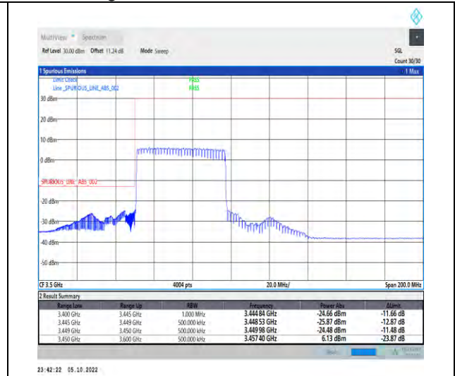
1-N77-3450-3550-PC2-30-50-L-3-DFT-QPSK-Outer_Full-128@0-Ant1-1--PASS-see graph
