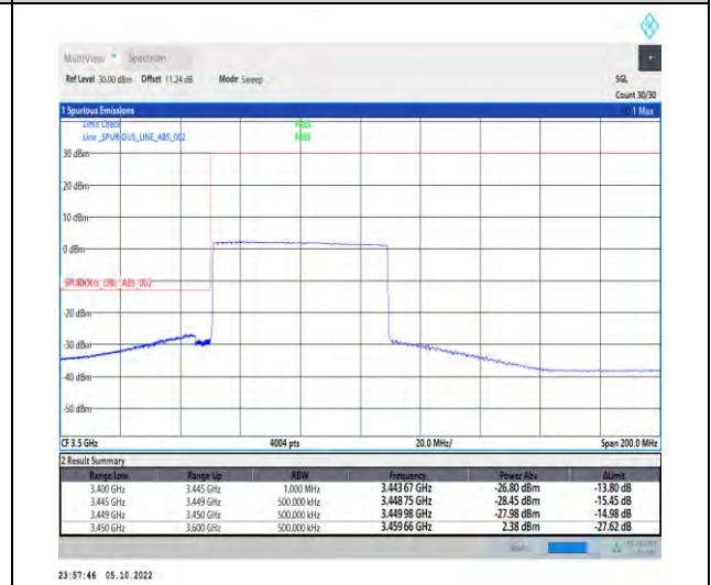
1-N77-3450-3550-PC2-30-60-L-6-CP-QPSK-Outer_Full-162@0-Ant1-1--PASS-see graph
