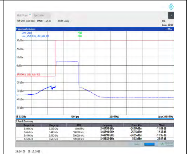
1-N77-3450-3550-PC2-30-30-L-6-CP-QPSK-Outer_Full-78@0-Ant1-1--PASS-see graph
