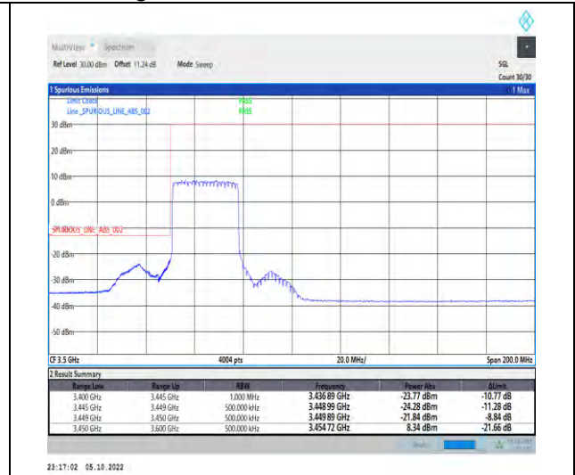
1-N77-3450-3550-PC2-30-30-L-3-DFT-QPSK-Outer_Full-75@0-Ant1-1--PASS-see graph
