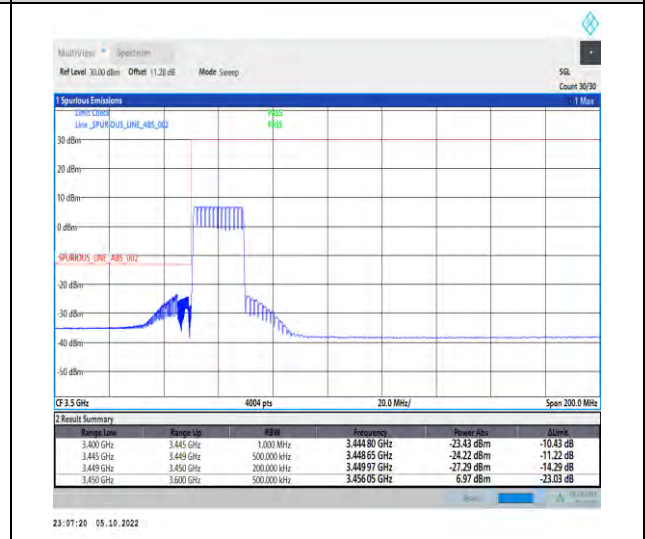
1-N77-3450-3550-PC2-30-20-L-6-CP-QPSK-Outer_Full-51@0-Ant1-1--PASS-see graph
