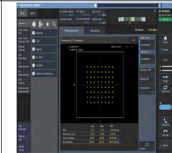
1-N77-3700-3980-PC2-30-100-M-8-CP-64QAM-Outer_Full-273@0-Ant1-see graph-PASS
