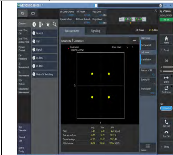
1-N77-3700-3980-PC2-30-100-M-6-CP-QPSK-Outer_Full-273@0-Ant1-see graph-PASS
