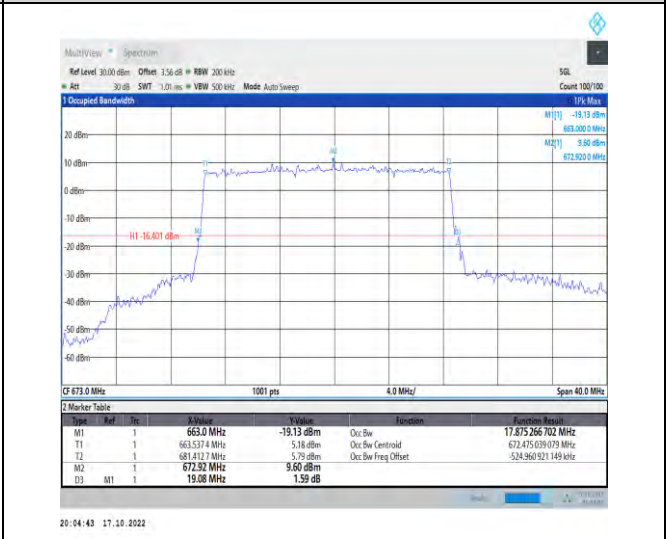
1-N71-PC3-15-20-L-5-DFT-256QAM-Outer_Full-100 @0-Ant1-17.875-19.080-≤20-PASS
