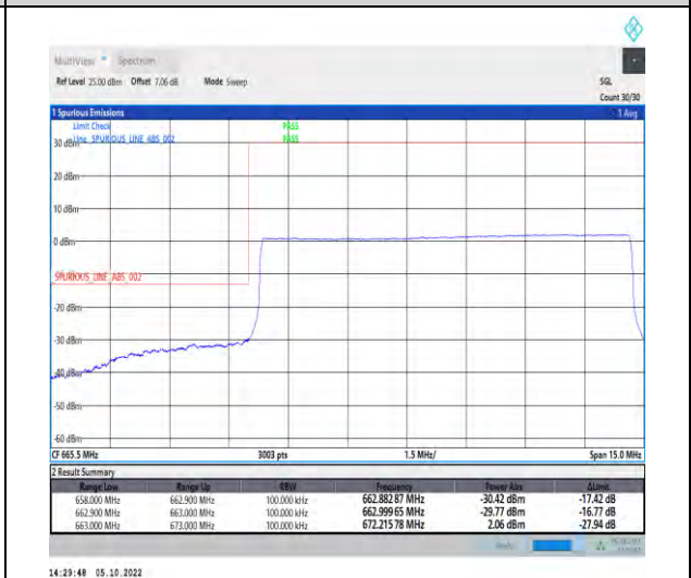
1-N71-PC3-15-10-L-6-CP-QPSK-Outer_Full-52@ 0-Ant1-1--PASS-see graph
