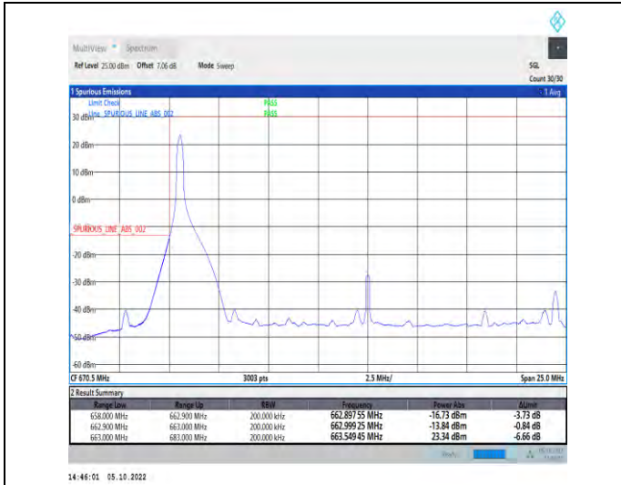
1-N71-PC3-15-20-L-1-DFT-QPSK-Edge_1RB_Left-1@ 0-Ant1-1--PASS-see graph
