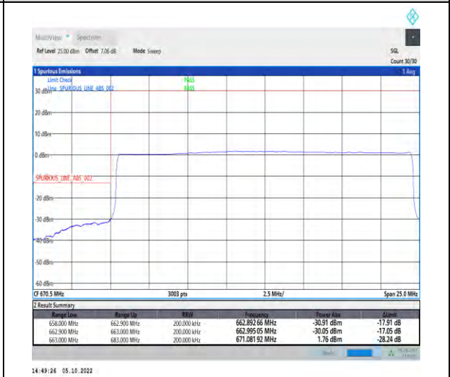
1-N71-PC3-15-20-L-6-CP-QPSK-Outer_Full-106 @0-Ant1-1--PASS-see graph
