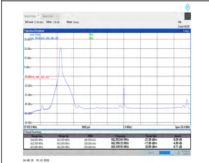
1-N71-PC3-15-20-L-4-CP-QPSK-Edge_1RB_Left-1@ 0-Ant1-1--PASS-see graph
