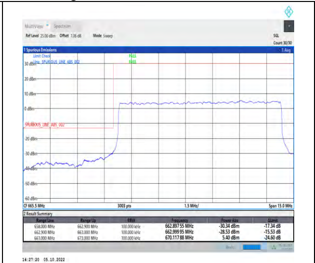
1-N71-PC3-15-10-L-3-DFT-QPSK-Outer_Full-50@ 0-Ant1-1--PASS-see graph
