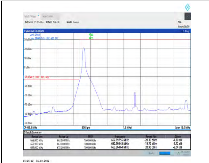
1-N71-PC3-15-10-L-1-DFT-QPSK-Edge_1RB_Left-1@ 0-Ant1-1--PASS-see graph
