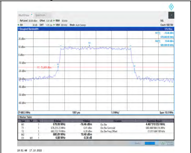
1-N71-PC3-15-5-M-7-CP-16QAM-Outer_Full-25@0-A nt1-4.468-4.880-<math>\leq</math>5-PASS
