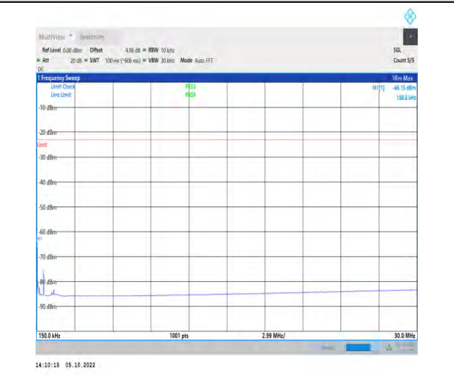
1-N71-PC3-15-20-M-1-DFT-QPSK-Inner_1RB_Left-1 @1-0.15-30-Ant1-0.15--66.15--23-PASS
