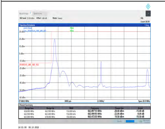
1-N71-PC3-15-15-L-4-CP-QPSK-Edge_1RB_Left-1@0 -Ant1-1--PASS-see graph
