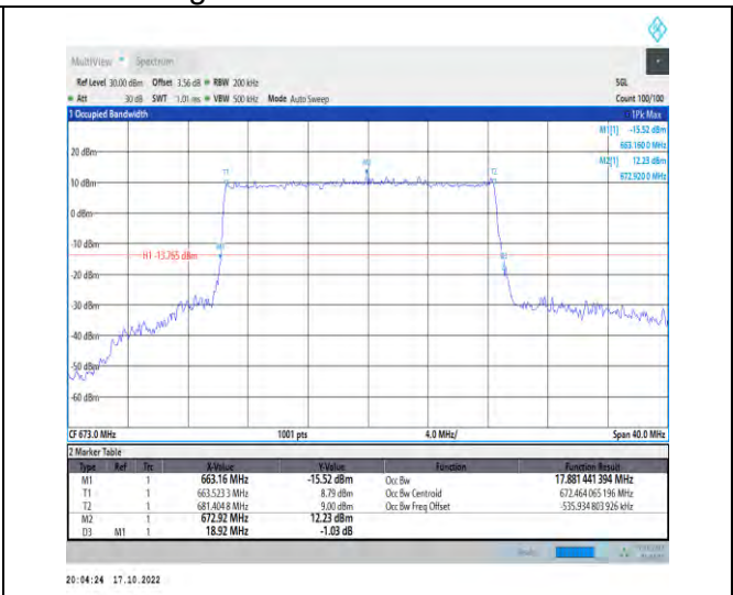
1-N71-PC3-15-20-L-3-DFT-16QAM-Outer_Full-100@ 0-Ant1-17.881-18.920-≤20-PASS
