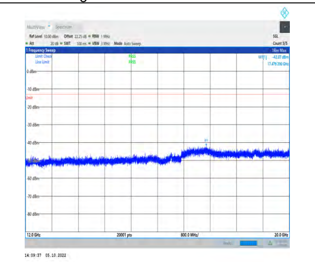
1-N71-PC3-15-20-L-1-DFT-QPSK-Inner_1RB_Left-1 @1-12000-20000-Ant1-17479.20--42.07--13-PASS
