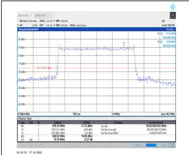
1-N71-PC3-15-20-H-6-CP-QPSK-Outer_Full-106@0 -Ant1-18.953-19.760-≤20-PASS
