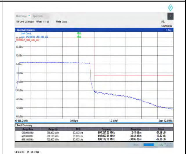
1-N71-PC3-15-5-H-6-CP-QPSK-Outer_Full-25@0- Ant1-1--PASS-see graph
