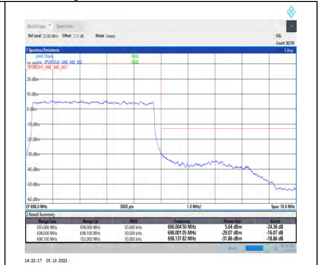
1-N71-PC3-15-5-H-3-DFT-QPSK-Outer_Full-25@ 0-Ant1-1--PASS-see graph
