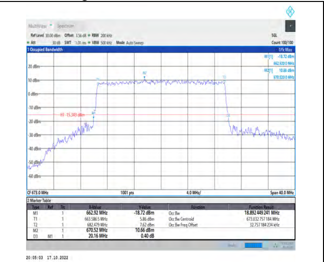
1-N71-PC3-15-20-L-7-CP-16QAM-Outer_Full-106@0 -Ant1-18.892-20.160-≤20-PASS
