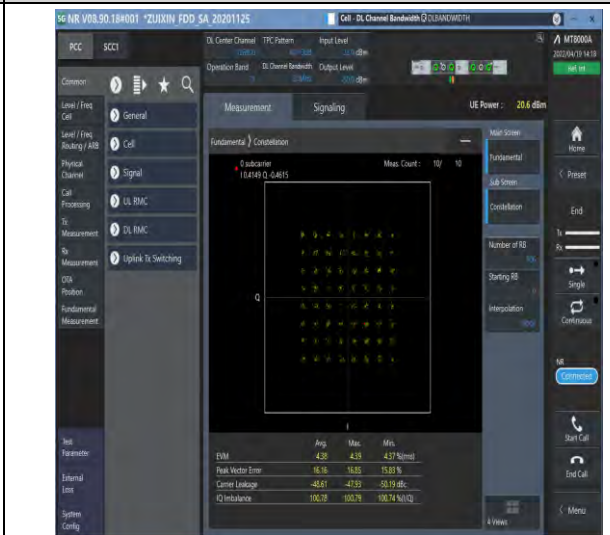
1-N71--15-20-M-8-CP-64QAM-Outer_Full-106@0-Ant1-see graph-PASS
