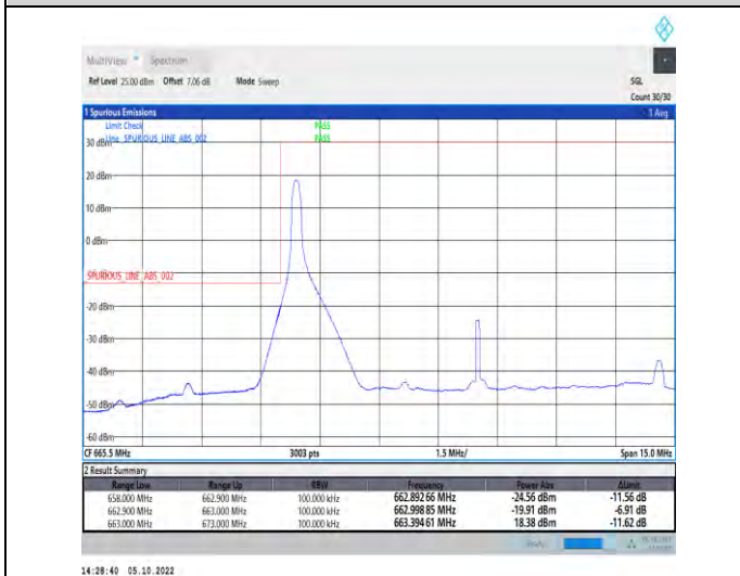
1-N71-PC3-15-10-L-4-CP-QPSK-Edge_1RB_Left-1@0 -Ant1-1--PASS-see graph
