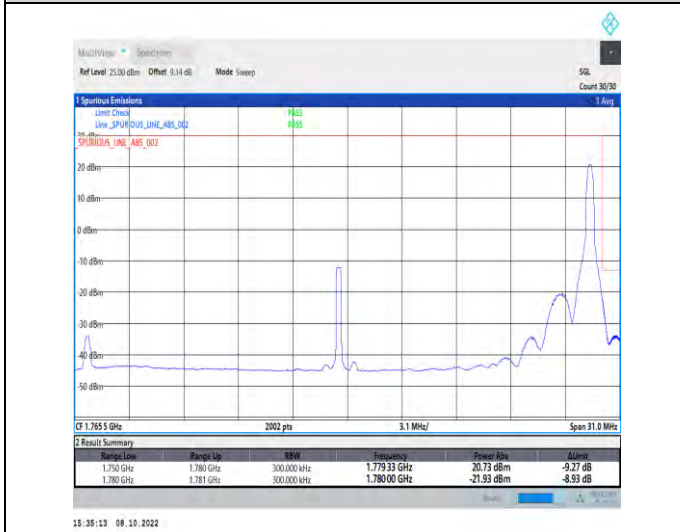
1-N66-PC3-15-30-H-5-CP-QPSK-Edge_1RB_Right-1 @159-Ant1-1-seegraph-PASS-see graph
