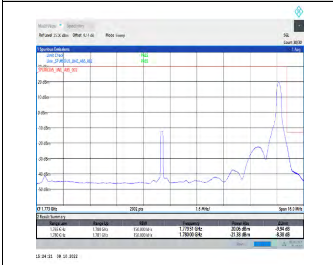
1-N66-PC3-15-15-H-5-CP-QPSK-Edge_1RB_Right-1 @78-Ant1-1-seegraph-PASS-see graph
