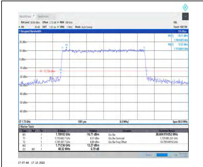
1-N66-PC3-15-40-L-6-CP-QPSK-Outer_Full-216@0 -Ant1-38.605-40.320-≤40-PASS
