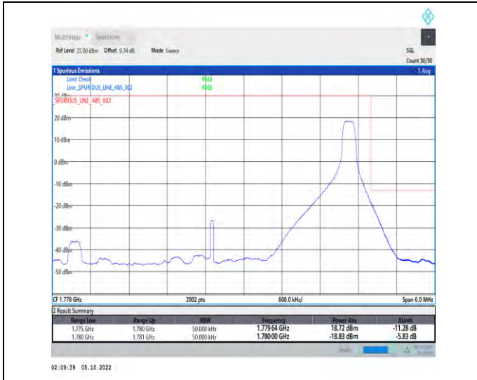
1-N66-PC3-15-5-H-2-DFT-QPSK-Edge_1RB_Right-1 @24-Ant1-1-seegraph-PASS-see graph
