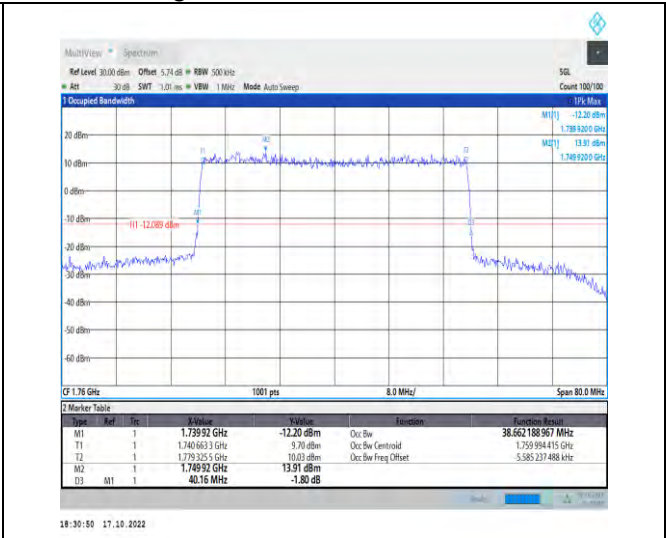
1-N66-PC3-15-40-H-3-DFT-16QAM-Outer_Full-216 @0-Ant1-38.662-40.160-≤40-PASS
