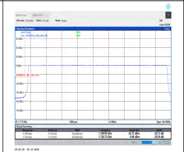
1-N66-PC3-15-15-L-6-CP-QPSK-Outer_Full-79@0-Ant1-1-seegraph-PASS-see graph
