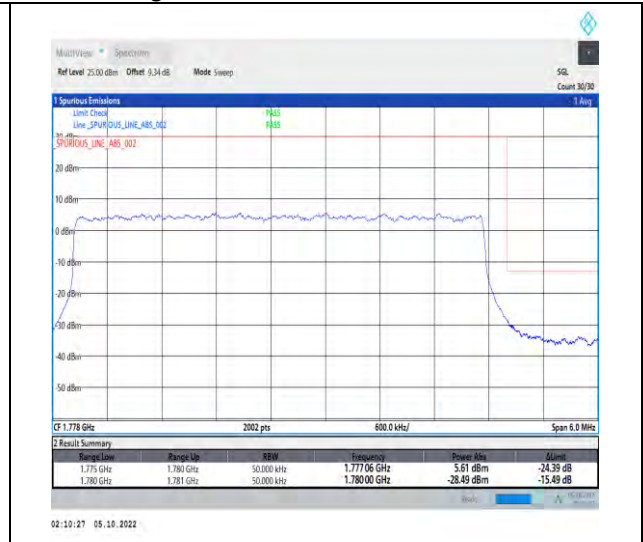
1-N66-PC3-15-5-H-3-DFT-QPSK-Outer_Full-25@0-Ant1-1-seegraph-PASS-see graph
