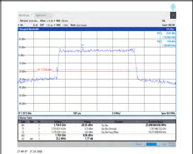
1-N66-PC3-15-25-H-9-CP-256QAM-Outer_Full-133@0-Ant1-23.699-25.200-≤25-PASS
