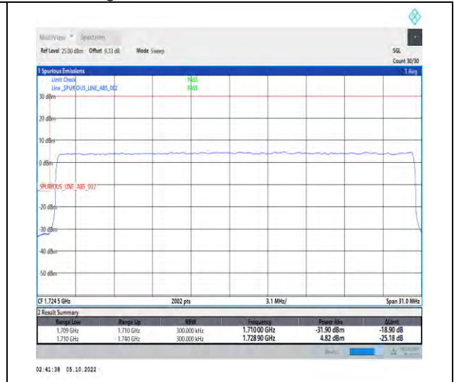
1-N66-PC3-15-30-L-3-DFT-QPSK-Outer_Full-160@0-Ant1-1-seegraph-PASS-see graph
