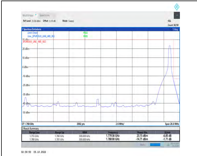
1-N66-PC3-15-25-H-2-DFT-QPSK-Edge_1RB_Right-1 @132-Ant1-1-seegraph-PASS-see graph
