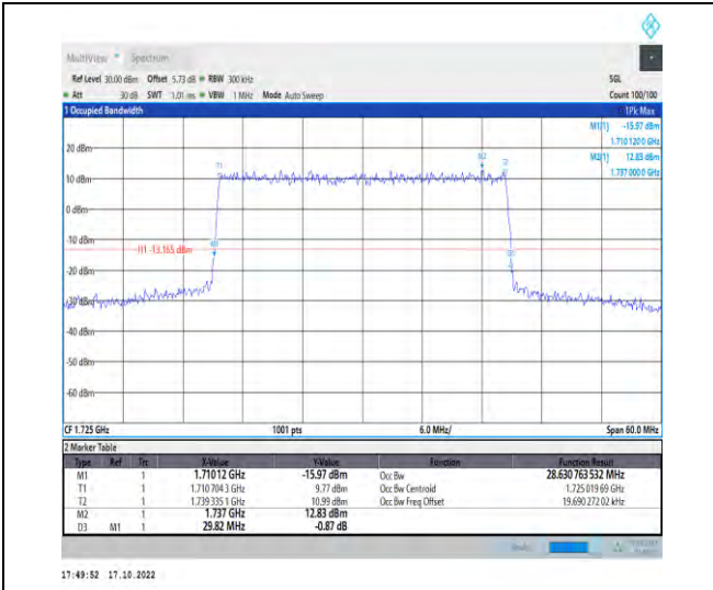
1-N66-PC3-15-30-L-1-DFT-QPSK-Outer_Full-160@ 0-Ant1-28.631-29.820-≤30-PASS
