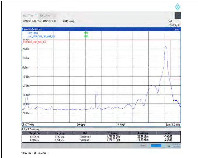
1-N66-PC3-15-15-H-2-DFT-QPSK-Edge_1RB_Right-1 @78-Ant1-1-seegraph-PASS-see graph
