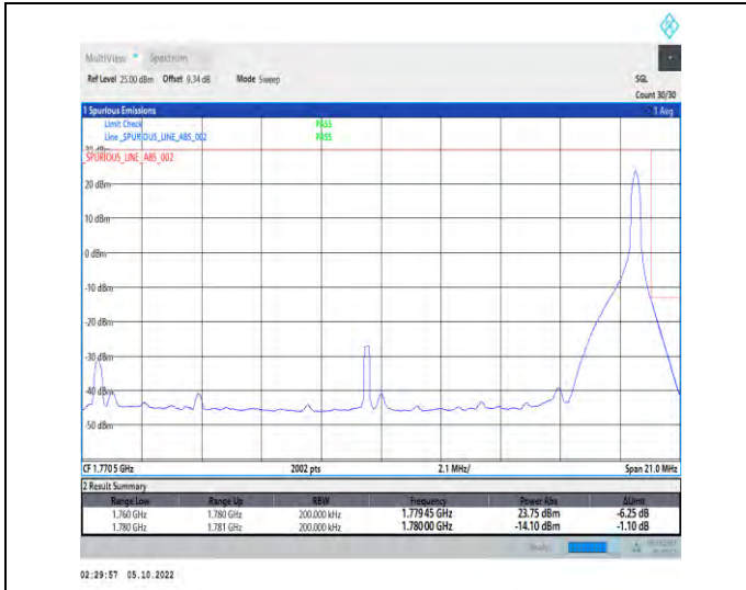
1-N66-PC3-15-20-H-2-DFT-QPSK-Edge_1RB_Right-1 @105-Ant1-1-seegraph-PASS-see graph
