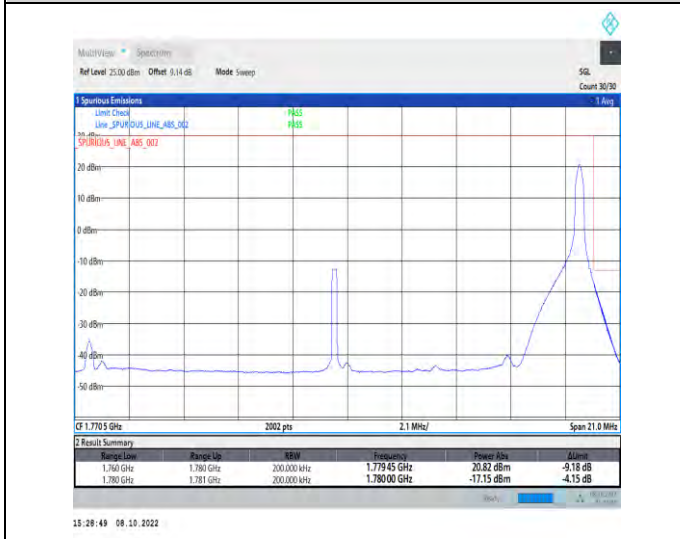
1-N66-PC3-15-20-H-5-CP-QPSK-Edge_1RB_Right-1 @105-Ant1-1-seegraph-PASS-see graph
