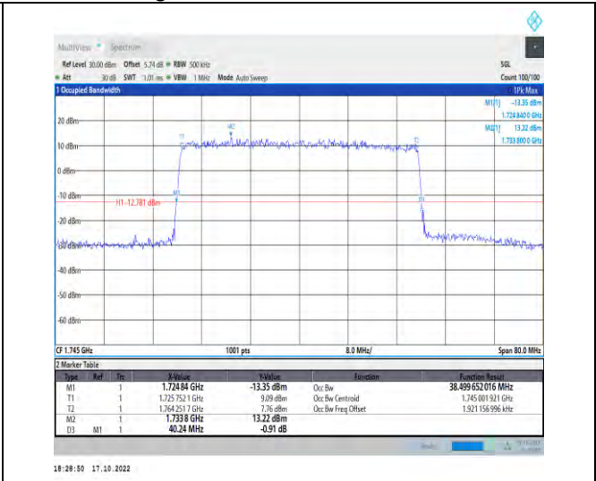
1-N66-PC3-15-40-M-3-DFT-16QAM-Outer_Full-216 @0-Ant1-38.5-40.240-≤40-PASS
