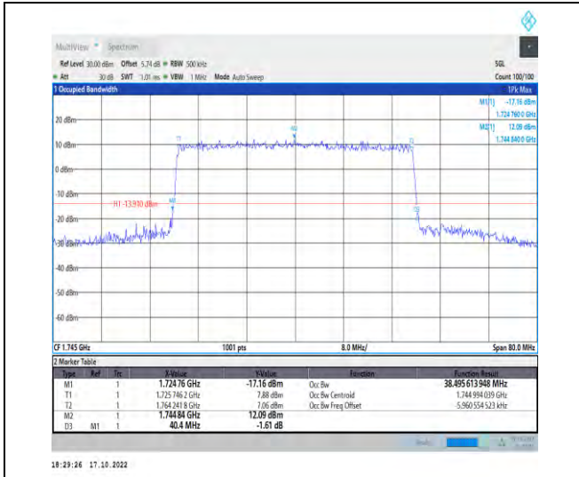
1-N66-PC3-15-40-M-6-CP-QPSK-Outer_Full-216@0 -Ant1-38.496-40.400-≤40-PASS
