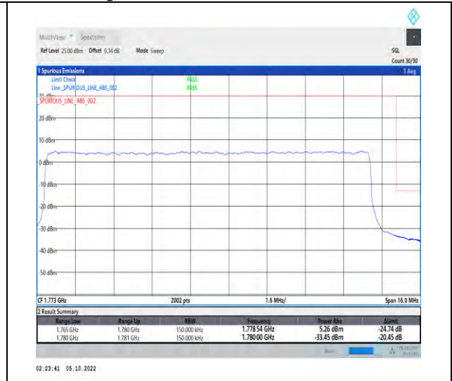
1-N66-PC3-15-15-H-3-DFT-QPSK-Outer_Full-75 @0-Ant1-1-seegraph-PASS-see graph
