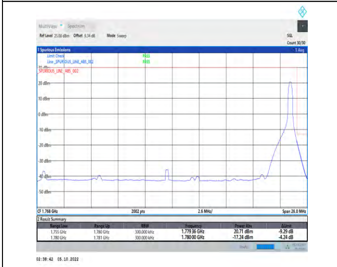
1-N66-PC3-15-25-H-5-CP-QPSK-Edge_1RB_Right-1 @132-Ant1-1-seegraph-PASS-see graph
