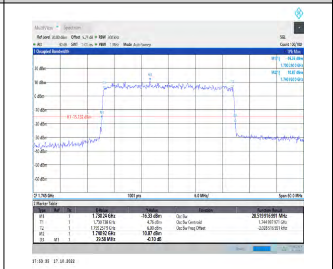
1-N66-PC3-15-30-M-5-DFT-256QAM-Outer_Full-160 @0-Ant1-28.52-29.580-≤30-PASS
