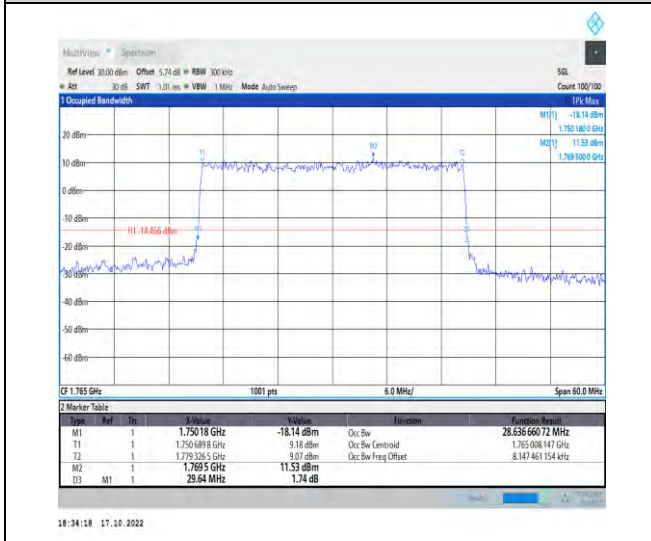
1-N66-PC3-15-30-H-4-DFT-64QAM-Outer_Full-160 @0-Ant1-28.637-29.640-≤30-PASS
