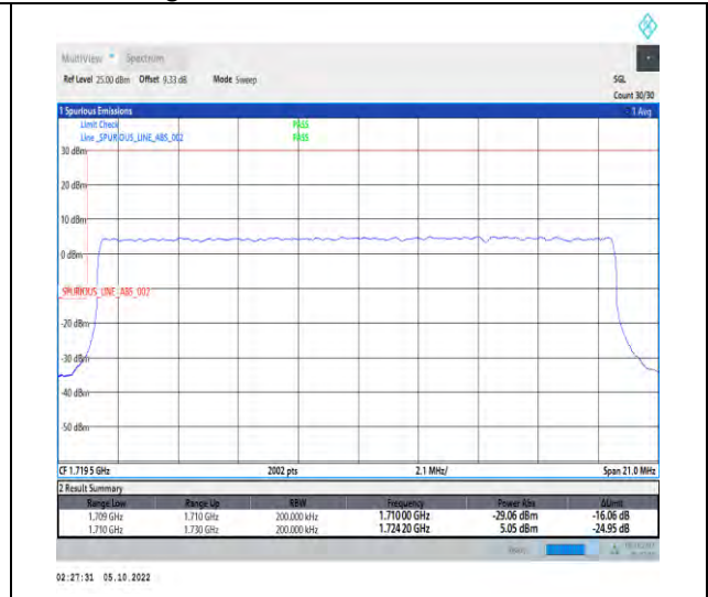
1-N66-PC3-15-20-L-3-DFT-QPSK-Outer_Full-100@0-Ant1-1-seegraph-PASS-see graph
