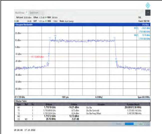
1-N66-PC3-15-30-L-4-DFT-64QAM-Outer_Full-160 @0-Ant1-28.631-29.760-≤30-PASS
