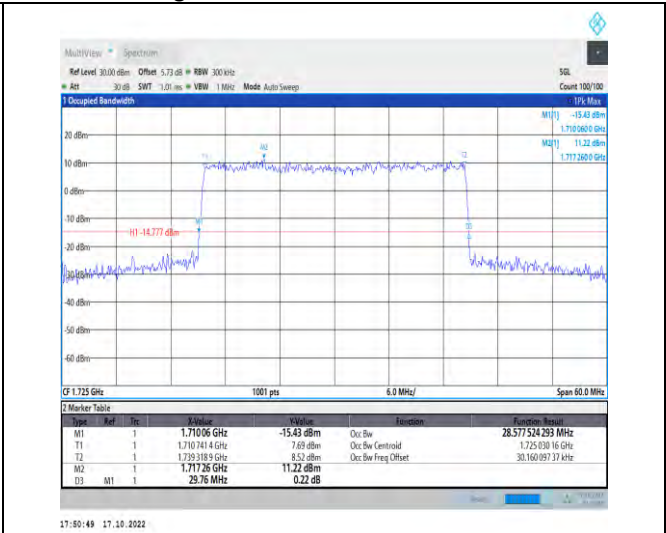
1-N66-PC3-15-30-L-7-CP-16QAM-Outer_Full-160@0 -Ant1-28.578-29.760-≤30-PASS
