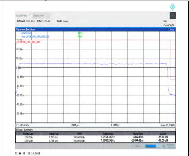
1-N66-PC3-15-30-H-3-DFT-QPSK-Outer_Full-160 @0-Ant1-1-seegraph-PASS-see graph
