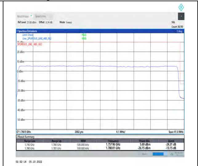
1-N66-PC3-15-40-H-3-DFT-QPSK-Outer_Full-216 @0-Ant1-1-seegraph-PASS-see graph
