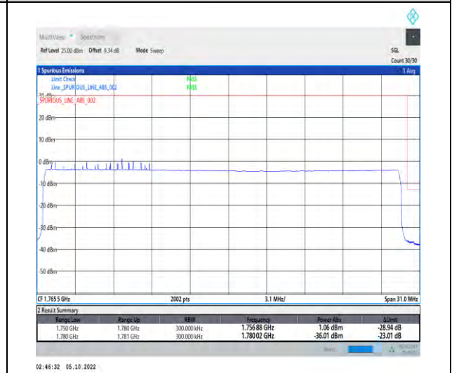
1-N66-PC3-15-30-H-6-CP-QPSK-Outer_Full-160 @0-Ant1-1-seegraph-PASS-see graph
