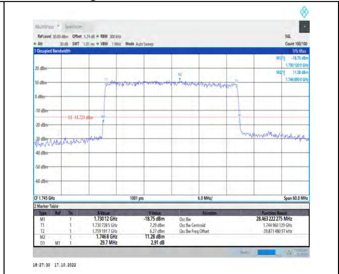
1-N66-PC3-15-30-M-3-DFT-16QAM-Outer_Full-160 @0-Ant1-28.463-29.700-≤30-PASS
