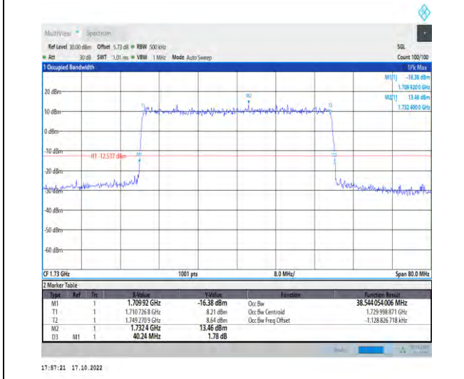
1-N66-PC3-15-40-L-4-DFT-64QAM-Outer_Full-216@0-Ant1-38.544-40.240-≤40-PASS
