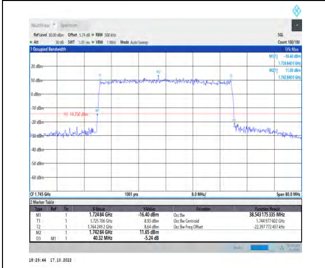
1-N66-PC3-15-40-M-8-CP-64QAM-Outer_Full-216 @0-Ant1-38.543-40.320-≤40-PASS
