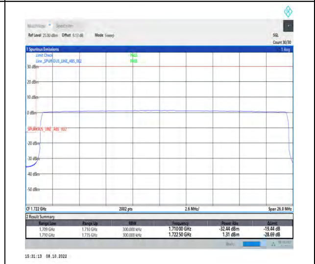
1-N66-PC3-15-25-L-6-CP-QPSK-Outer_Full-133@0-Ant1-1-seegraph-PASS-see graph
