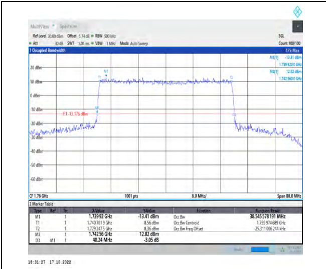
1-N66-PC3-15-40-H-6-CP-QPSK-Outer_Full-216@0 -Ant1-38.546-40.240-≤40-PASS
