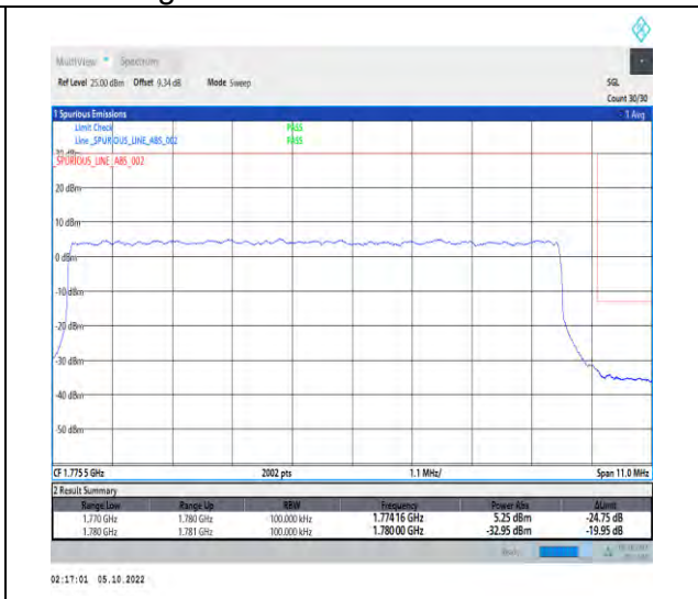
1-N66-PC3-15-10-H-3-DFT-QPSK-Outer_Full-50 @0-Ant1-1-seegraph-PASS-see graph
