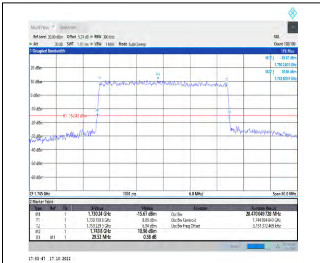
1-N66-PC3-15-30-M-6-CP-QPSK-Outer_Full-160@0 -Ant1-28.47-29.520-≤30-PASS
