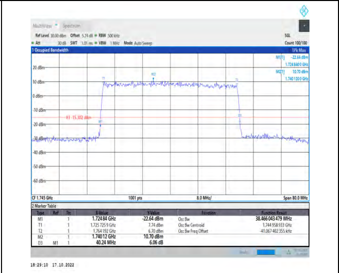
1-N66-PC3-15-40-M-5-DFT-256QAM-Outer_Full-216 @0-Ant1-38.466-40.240-≤40-PASS
