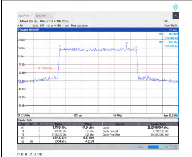
1-N66-PC3-15-30-L-8-CP-64QAM-Outer_Full-160@0 -Ant1-28.521-29.580-≤30-PASS
