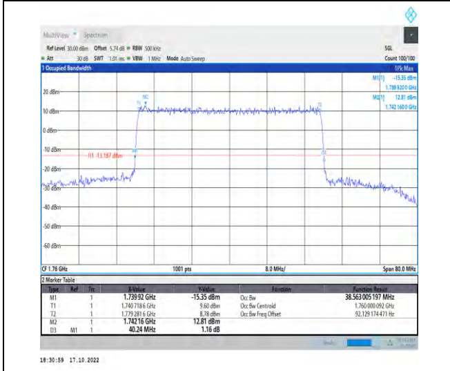
1-N66-PC3-15-40-H-4-DFT-64QAM-Outer_Full-216 @0-Ant1-38.563-40.240-≤40-PASS
