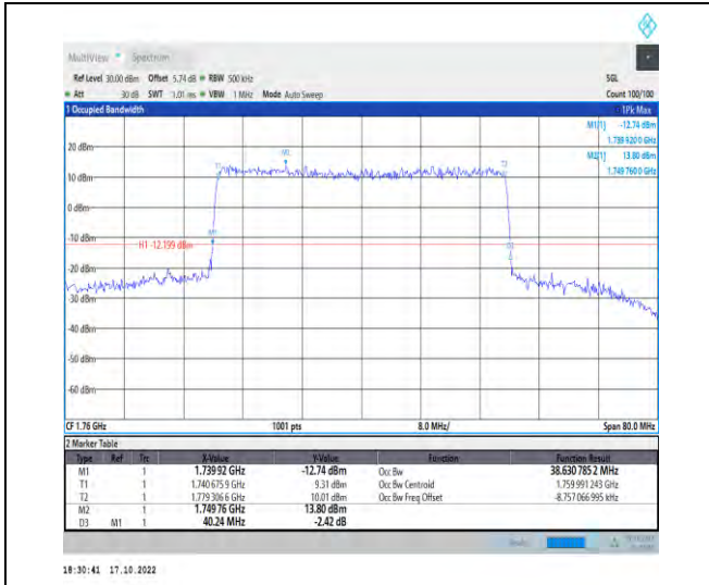
1-N66-PC3-15-40-H-1-DFT-QPSK-Outer_Full-216@ 0-Ant1-38.631-40.240-≤40-PASS
