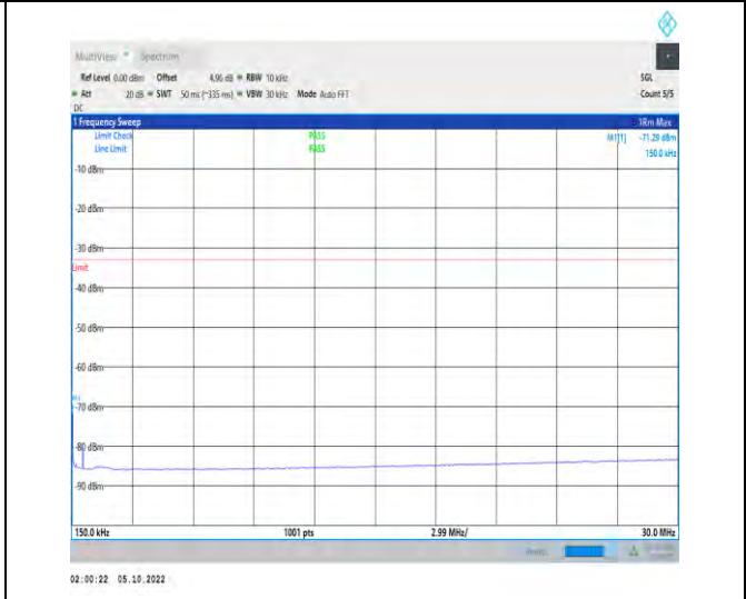
1-N66-PC3-15-40-M-1-DFT-QPSK-Inner_1RB_Left-1 @1-0.15-30-Ant1-0.15--71.29--33-PASS
