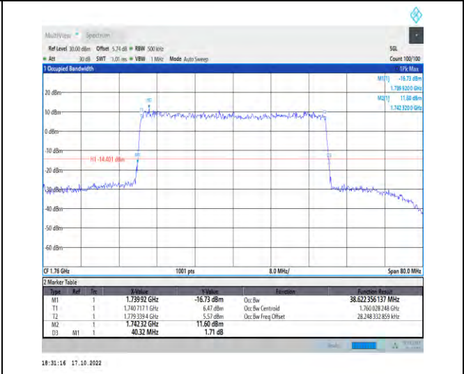
1-N66-PC3-15-40-H-5-DFT-256QAM-Outer_Full-216 @0-Ant1-38.622-40.320-≤40-PASS
