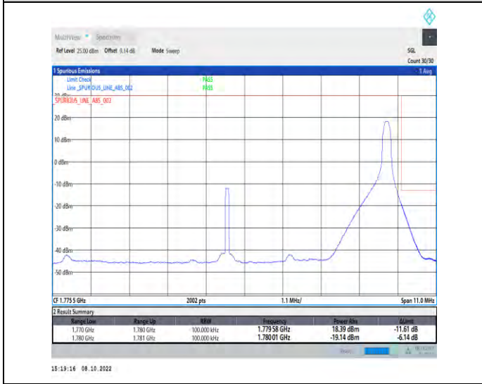
1-N66-PC3-15-10-H-5-CP-QPSK-Edge_1RB_Right-1 @51-Ant1-1-seegraph-PASS-see graph
