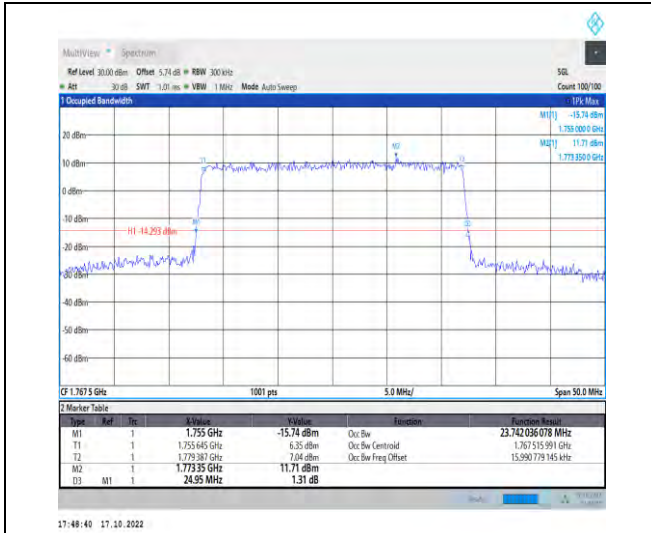
1-N66-PC3-15-25-H-6-CP-QPSK-Outer_Full-133@0 -Ant1-23.742-24.950-≤25-PASS
