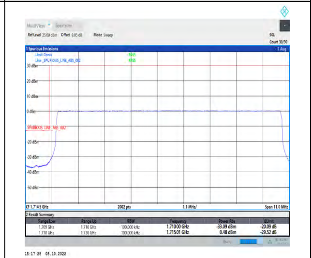
1-N66-PC3-15-10-L-6-CP-QPSK-Outer_Full-52@0-Ant1-1-seegraph-PASS-see graph
