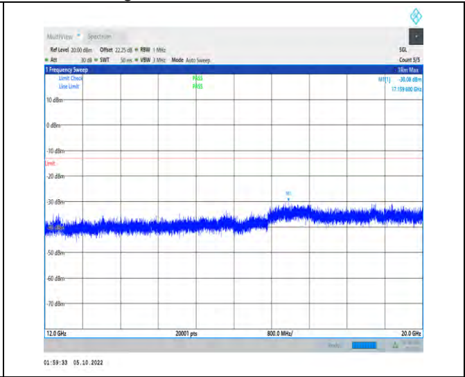
1-N66-PC3-15-40-L-1-DFT-QPSK-Inner_1RB_Left-1 @1-12000-20000-Ant1-17159.60--30.08--13-PASS
