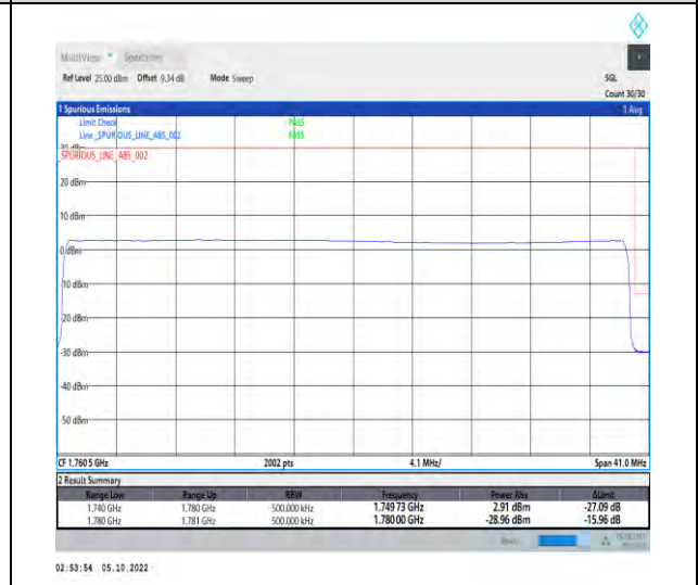
1-N66-PC3-15-40-H-6-CP-QPSK-Outer_Full-216 @0-Ant1-1-seegraph-PASS-see graph
